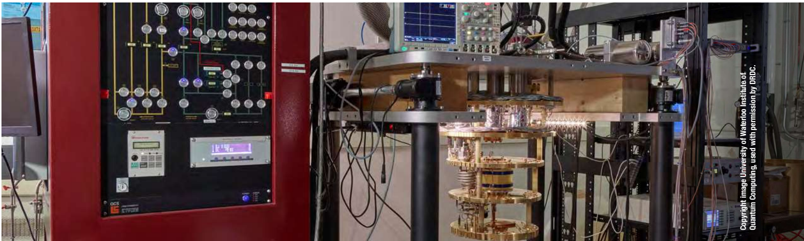
The Leiden CF1400 dilution refrigerator at the University of Waterloo Institute of Quantum Computing provides an ultra-low temperature platform for developing quantum devices.
