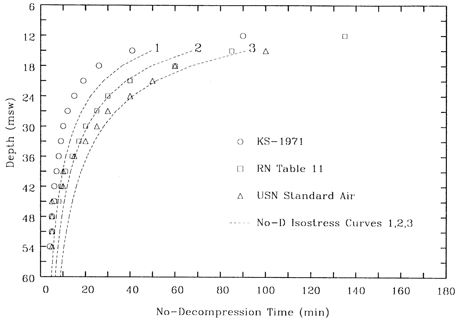
Fig. 2. Comparison of the KS-1971 no-decompression limits with those of the Royal Navy, US Navy, and the DCIEM no-decompression isostress curves.
