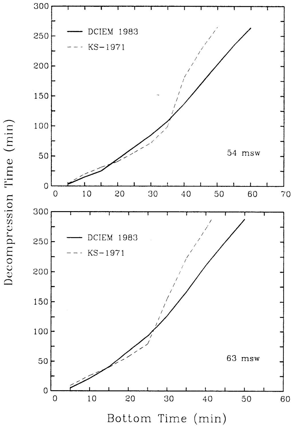
Fig. 5c. Comparison of DCIEM 1983 total decompression times for standard air dives with those of the Kidd-Stubbs (KS) 1971 model for 54 and 63 msw.
