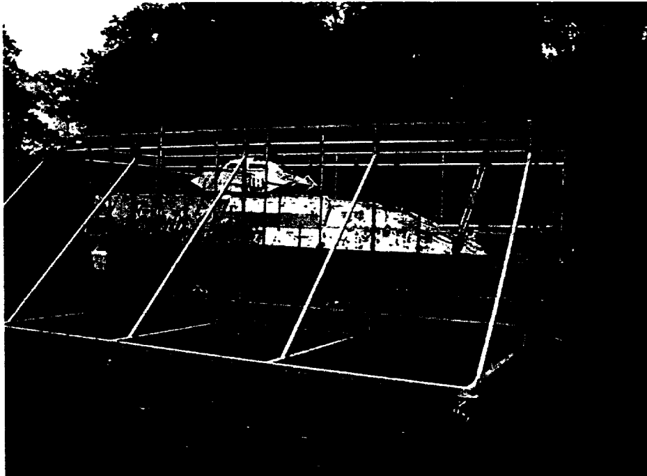
Figure 1. The ETBS cage for measuring vehicular contamination. Seventy-seven Geiger tubes are suspended from the metal structure; when the cage is closed around the vehicle, these tubes are within a few centimetres of the vehicle surface.
