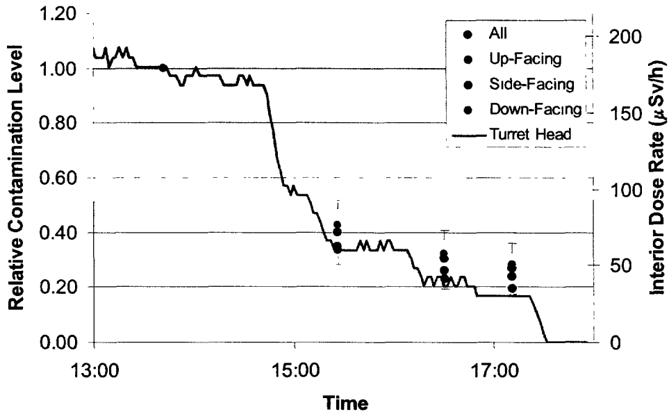
Figure 8. As in the previous figure, but now the line is for a dosimeter at the head position in the turret.
