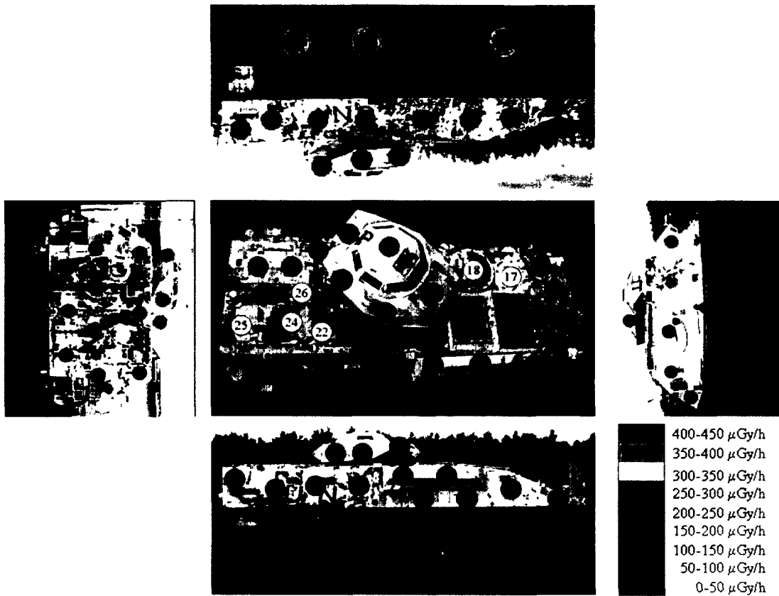
Figure 3. Contamination levels measured with the Geiger tube cage immediately after contamination.
