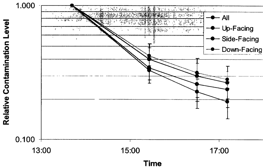
Figure 6. Relative contamination levels (according to Geiger tube readings) as a function of time. The 77 Geiger tube readings are grouped into 3 regions, shown in the legend. The overall averages are also shown. The error bars are standard deviations for the distributions.
