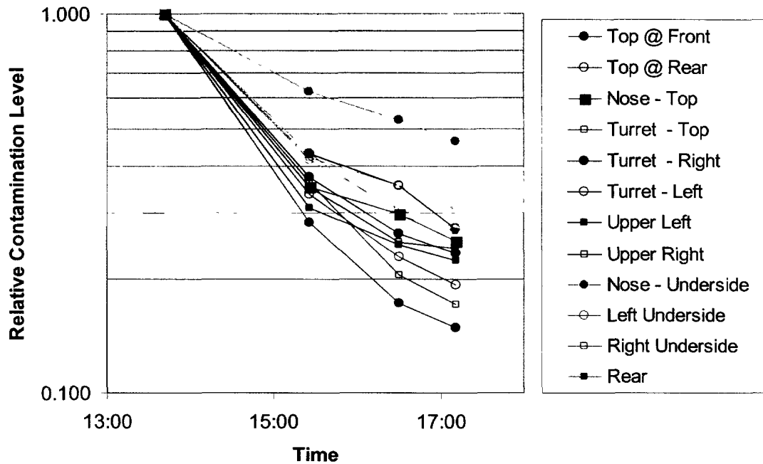
Figure 5. Relative contamination levels (according to Geiger tube readings) as a function of time. The 77 Geiger tube readings are grouped into 12 regions, shown in the legend. The four measurement times denote the measurement following contamination and each of the measurements following the three decontamination attempts.
