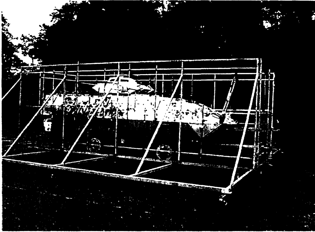
Figure 1. Measuring contamination levels with the ETBS cage. Seventy-seven Geiger tubes are suspended by the metal structure. The cage rides on wheels, allowing it to be rolled into place, enclosing the vehicle.
