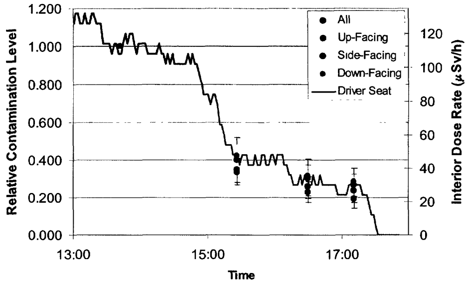
Figure 7. External and internal measurements of contamination. The data points are the contamination levels measured by the Geiger tube cage for each of the three surfaces defined in the previous section. The line is the dose rate measured by the dosimeter sitting on the driver's seat. The dosimeter dose rate falls to zero at 17:30 when the dosimeter when the dosimeter is removed from the vehicle.
