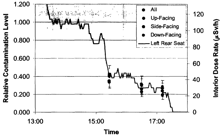
Figure 9. As in the previous figure, but now the line denotes the dose rate on the left passenger bench, near the rear of the vehicle.
