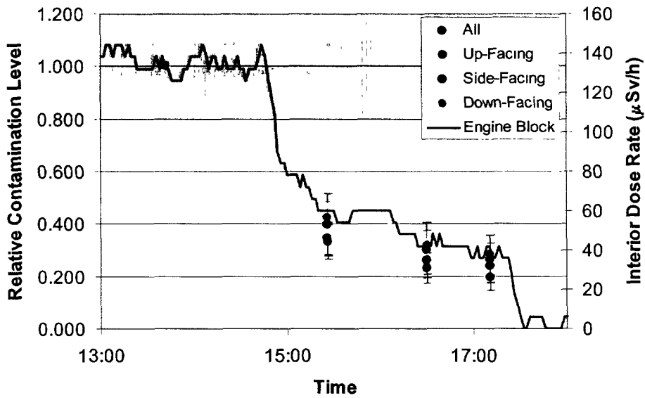
Figure 10. As in the previous figure, but now the line denotes the dose rate measured at waist height, immediately behind the engine compartment.
