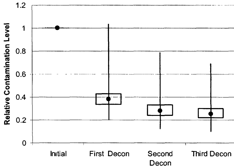
Figure 4. Box and whisker plot showing the relative contamination levels (according to measurements from the Geiger tube cage) on the vehicle after contamination and after each of the three phases of decontamination. In a box and whisker plot, the vertical line defines the maximum and minimum of the distribution, the box defines the upper and lower quartiles, and the circle denotes the median.
