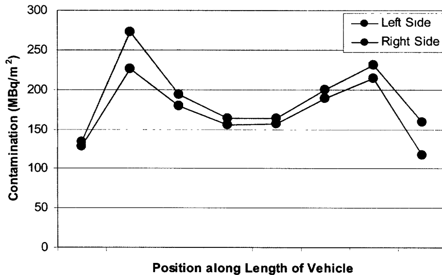
Figure 2. Contamination levels measured on the witness plates next to the Grizzly in the contamination area.
