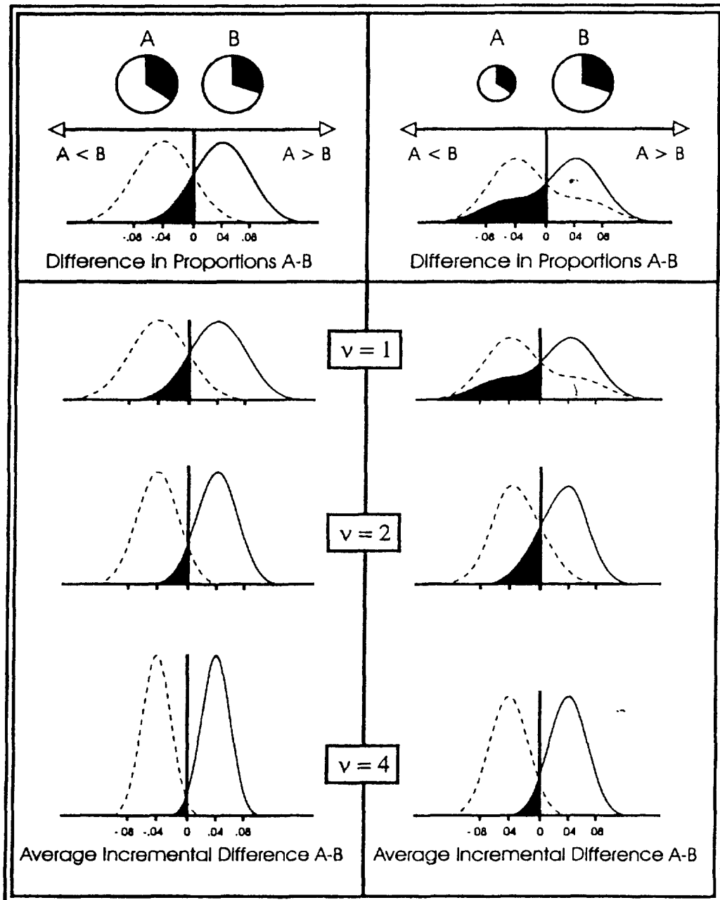
Figure 3 An illustration of the effect of repeated sampling in the incremental estimation model with equal sizes (Experiment 1) shown on the left and unequal sizes (Experiment 2) shown on the right. Note that error decreases with repeated sampling and that the distributions become more symmetric with repeated sampling in the unequal-size case
