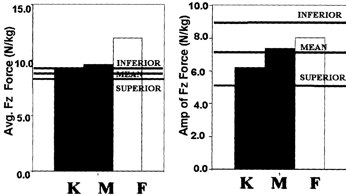
Figure 6a. Average Force (Fz) from the LC Simulator. Figure 6b. Amplitude of Force (Fz) from the LC Simulator.
