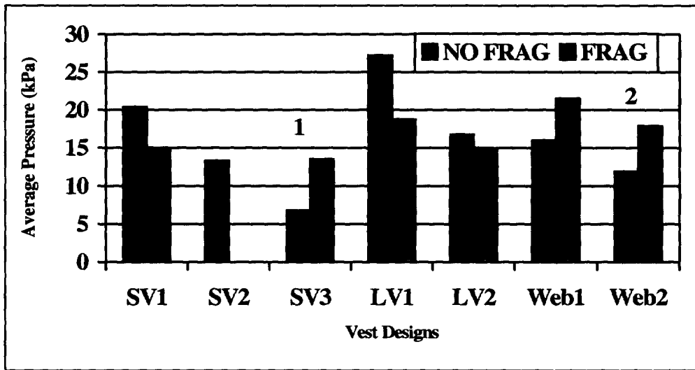
Figure 4. Effect of Tactical Vest Designs on Average Shoulder Pressure
