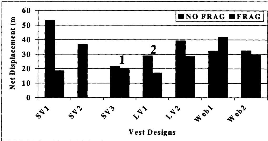
Figure 3. Effect of Tactical Vest Designs on Net Relative Kit Displacement
