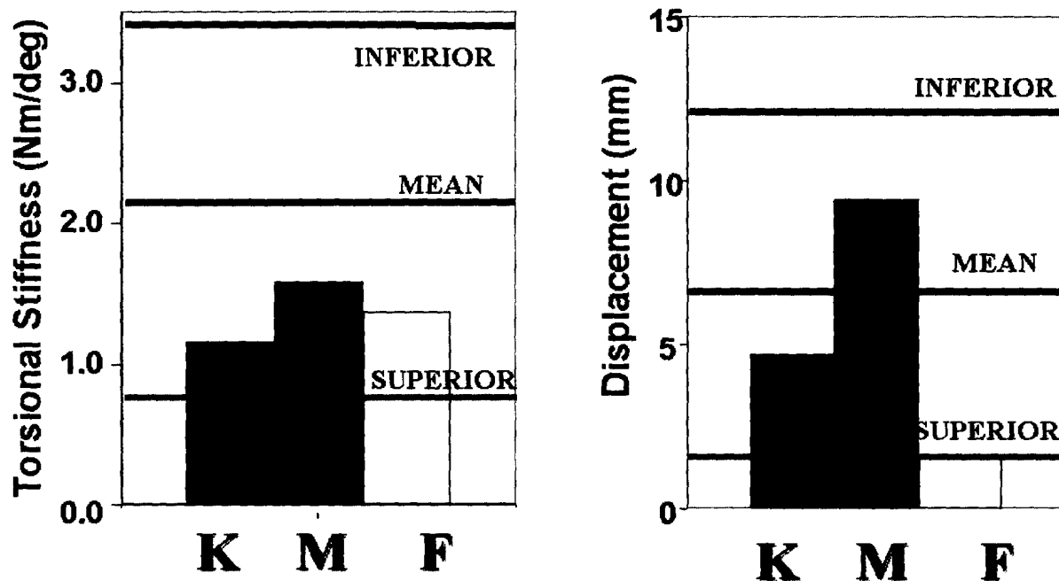
Figure 5a. Suspension Stiffness from the LC Compliance Tester. Figure 5b. Relative Pack Displacement from LC Simulator
