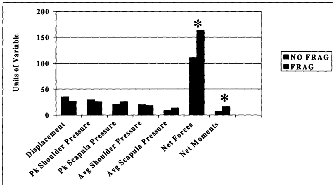
Figure 2. Effect of Wearing a Fragmentation Vest on LC Simulator Measures
