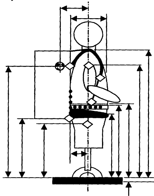
Figure 3. Schematic of Load Distribution Test Apparatus (Shoulder Strap attachment points indicated by black circles – 12 positions of varied vertical heights and horizontal positions. Optotrak position markers indicated by white diamonds).
