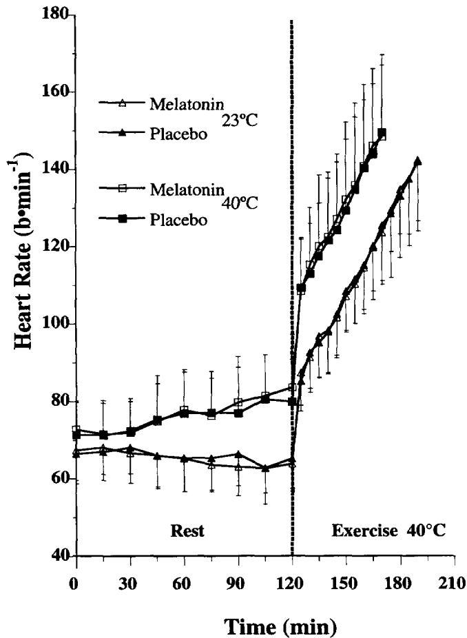
Fig. 1 Changes in heart rate during the 2 h rest at either 23 °C or 40 °C while wearing combat clothing and during subsequent exercise at 40 °C and 30% relative humidity while wearing the nuclear, biological and chemical protective ensemble. A 5 mg dose of melatonin or a placebo capsule was ingested after 30 min of rest. Values are mean and SD for n = 9 .
