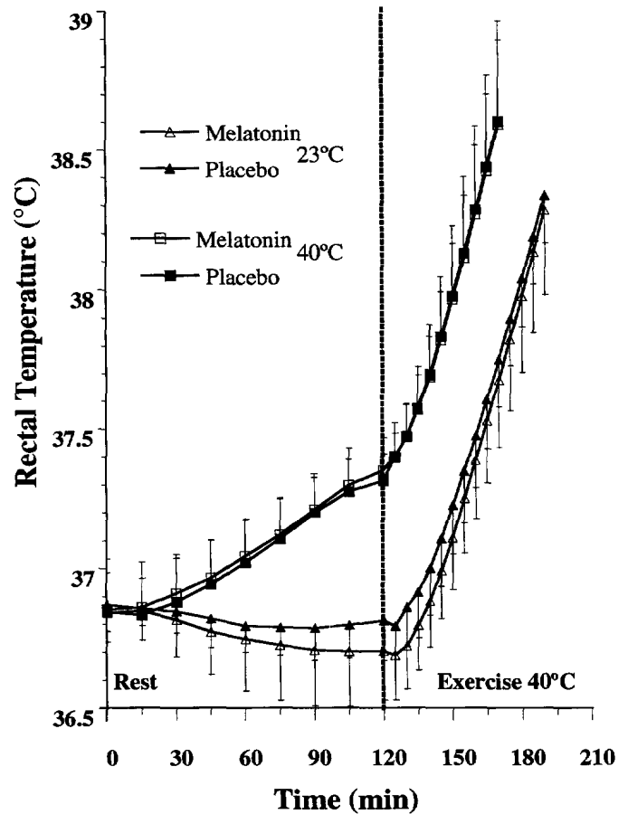
Fig. 2 Changes in rectal temperature during the 2 h rest period at either 23 °C or 40 °C while wearing combat clothing and during subsequent exercise at 40 °C and 30% relative humidity while wearing the nuclear, biological and chemical protective ensemble. A 5 mg dose of melatonin or a placebo capsule was ingested after 30 min of rest. Values are mean and SD for n = 9 .
