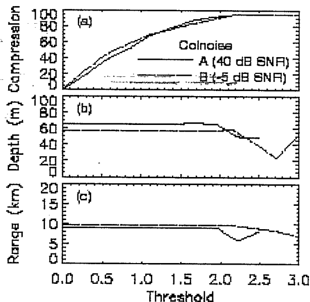
Figure 1. Matched field localization results using CSM with elements smaller than threshold set to zero. (a) sparse matrix compression percentage exclusive of additional reductions available from symmetry, (b) depth estimate, (c) range estimate.
