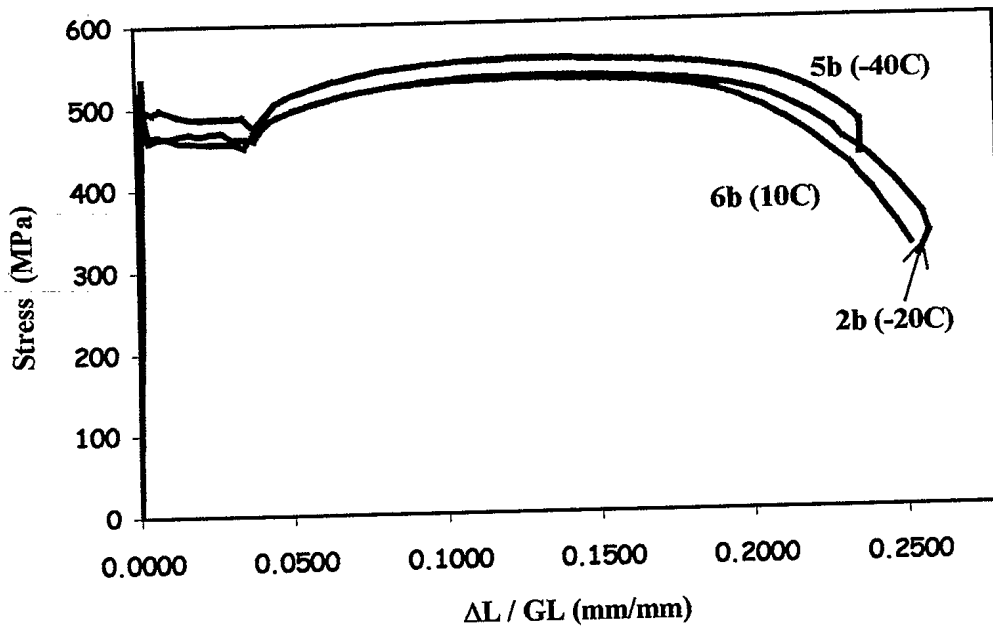
Figure 11. Two Inch Gauge Length Tensile Test Data.
