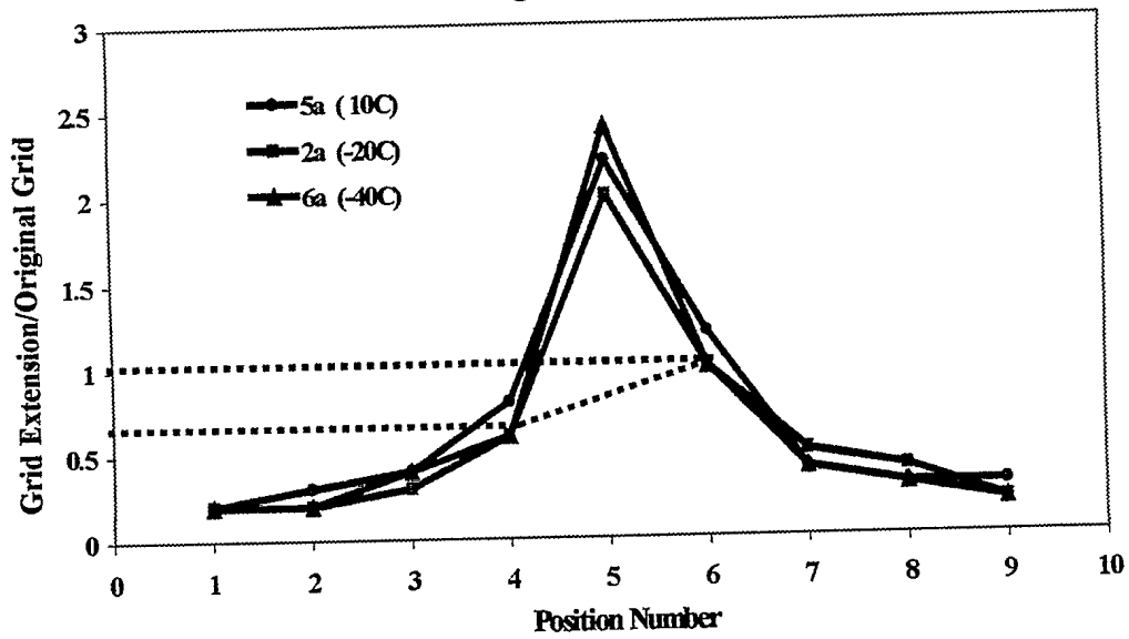
Figure 12a. One Inch Gauge Length Grid Extensions.
