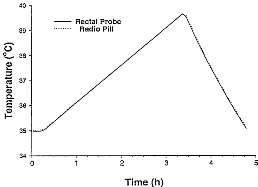
Figure 1. Plot of rectal probe and radio pill temperature curves as water bath is actively heated from 35 to 39.7°C and then allowed to passively cool.
