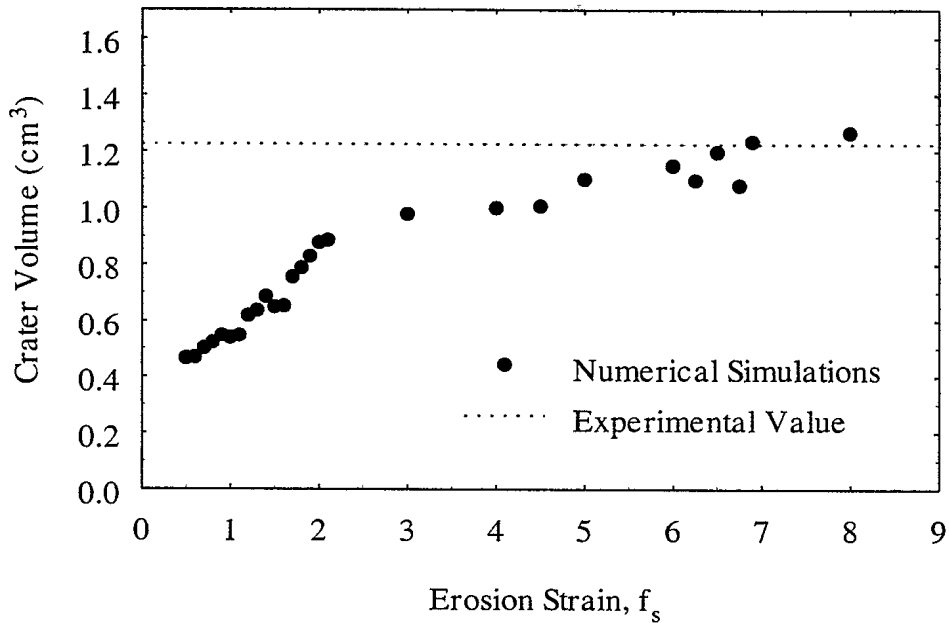
FIGURE 8 – Crater volume as a function of erosion strain for case of the 7.62-mm bullet penetrating a semi-infinite aluminium target
