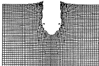
FIGURE 6 – Penetration/crater profile of the aluminium semi-infinite target struck by a M80 7.62-mm bullet at 817.5 m/s.
