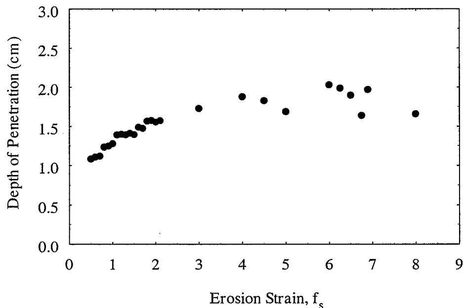
FIGURE 7 – Depth of penetration, DOP, as a function of erosion strain, f_s , for the case of a M80 7.62-mm striking a semi-infinite aluminium target
