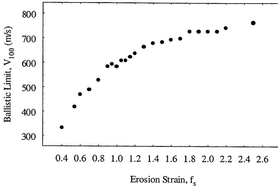
FIGURE 5 – Ballistic limit variation as a function of erosion strain, f_s , for the SS109 5.56-mm bullet/finite thickness target system
