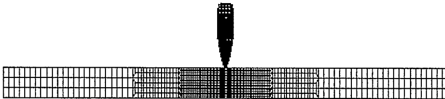
FIGURE 2 – SS109 5.56-mm bullet striking a 10.8-mm aluminium target
