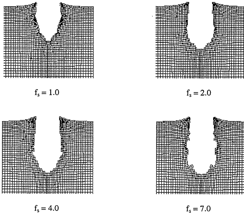
FIGURE 9 – Crater volume/shape comparison for four different erosion strains for the M80 7.62-mm projectile/semi-infinite aluminium target system
