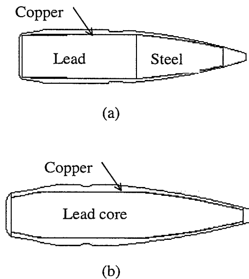
FIGURE 1 – Main features of the projectiles used in this study. (a) SS109 5.56-mm lead/steel core bullet, (b) M80 7.62-mm lead core bullet
