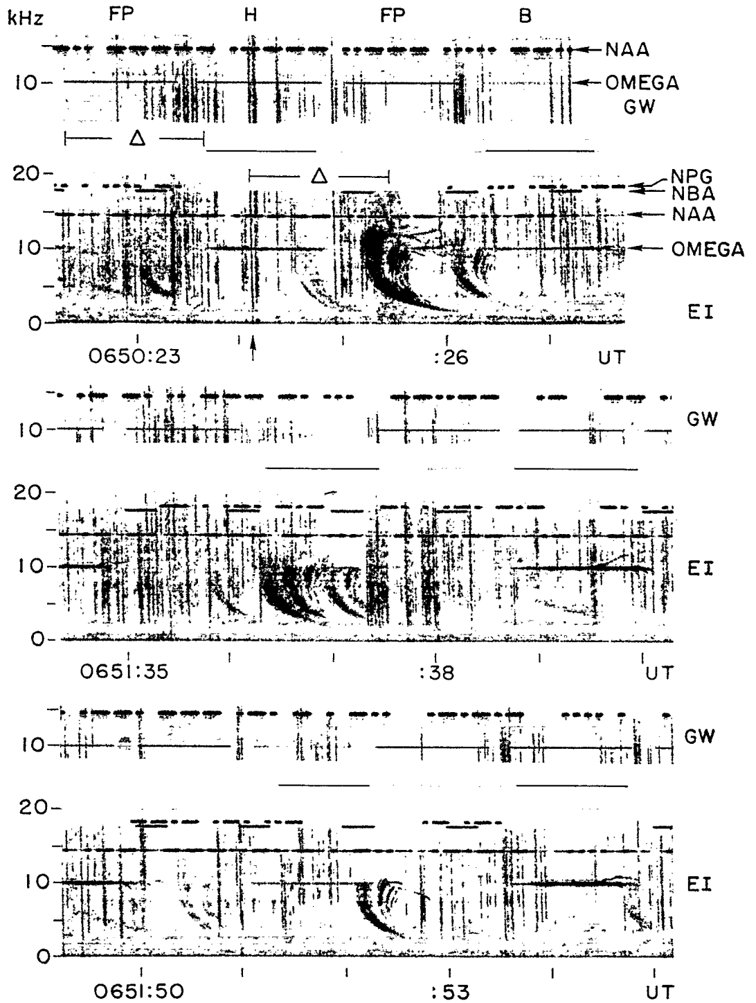
Fig. 8. Carpenter . Simultaneous conjugate recordings at Great Whale (GW) and Eights (EI), May 9, 1963, illustrating triggering of magnetospheric noise by \sim 1 -sec 10.2-kHz pulses from the low power ( \sim 100 watts) Omega transmitter at Forest Port, New York. See text for details.
