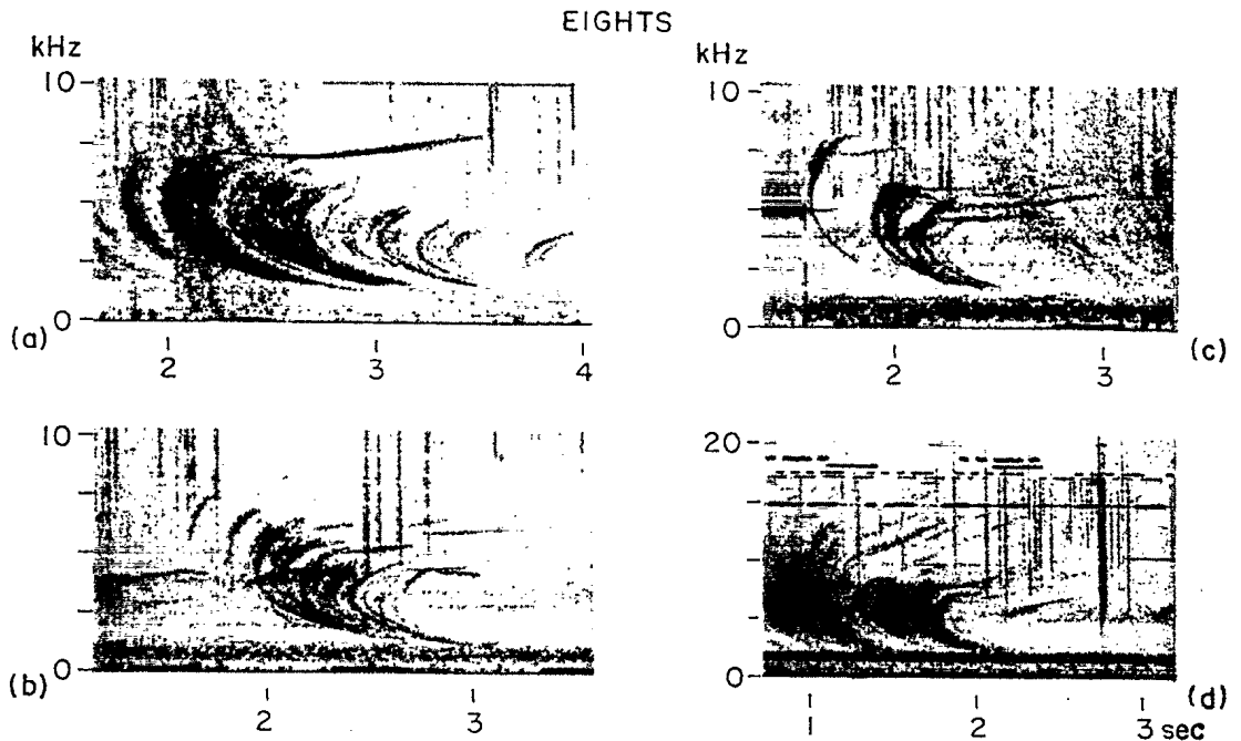
Fig. 1. Carpenter . Multicomponent whistlers illustrating the upper intensity cutoff. The spectra were recorded at Eights, Antarctica, during the synoptic intervals: June 6, 1963, 1450 UT (a); July 2, 1963, 1050 UT (b); July 2, 1963, 0950 UT (c); June 13, 1963, 1250 UT (d). The 5-kHz tone at the left in (c) is part of a system calibration. Case (d) is complicated by additional diffuse whistler activity in the background. Time is indicated in seconds from the causative atmospheric. Cases (a), (b), and (c) show the frequency band 0-10 kHz, case (d) shows 0-20 kHz.
