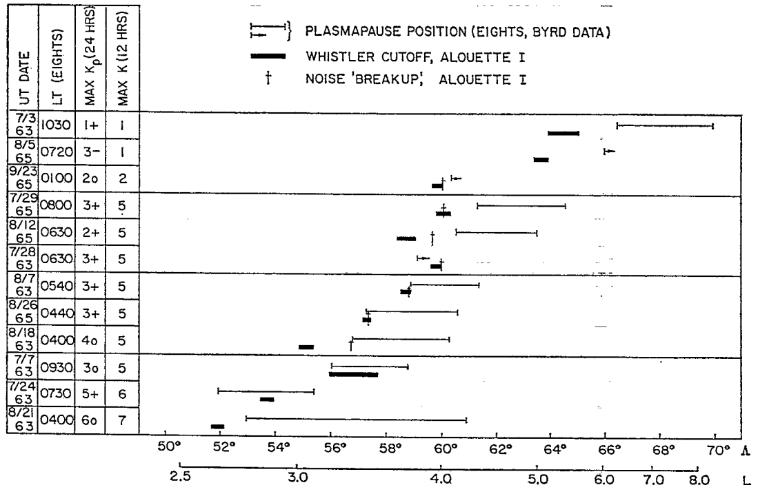
Fig. 3. Summary of case studies in which the whistler cutoff on Alouette 1 is compared with simultaneous ground measurements of the plasmapause position. The K values in the fourth column at the left are for Byrd Station. The systematic difference between the Alouette data and the ground measurements is discussed in the text.
