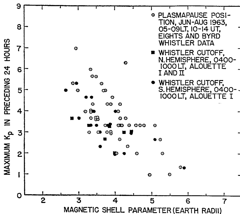
Fig. 4. A comparison of ground measurements of the plasmapause position with Alouette data on the whistler cutoff, both plotted in coordinates of maximum K_p in the preceding 24 hours versus a magnetic shell parameter. In the case of the whistler measurements, the parameter is approximate geocentric equatorial crossing in earth radii, whereas for the Alouette data it is L value calculated for 1000 km in the Jensen and Cain [1962] field.
