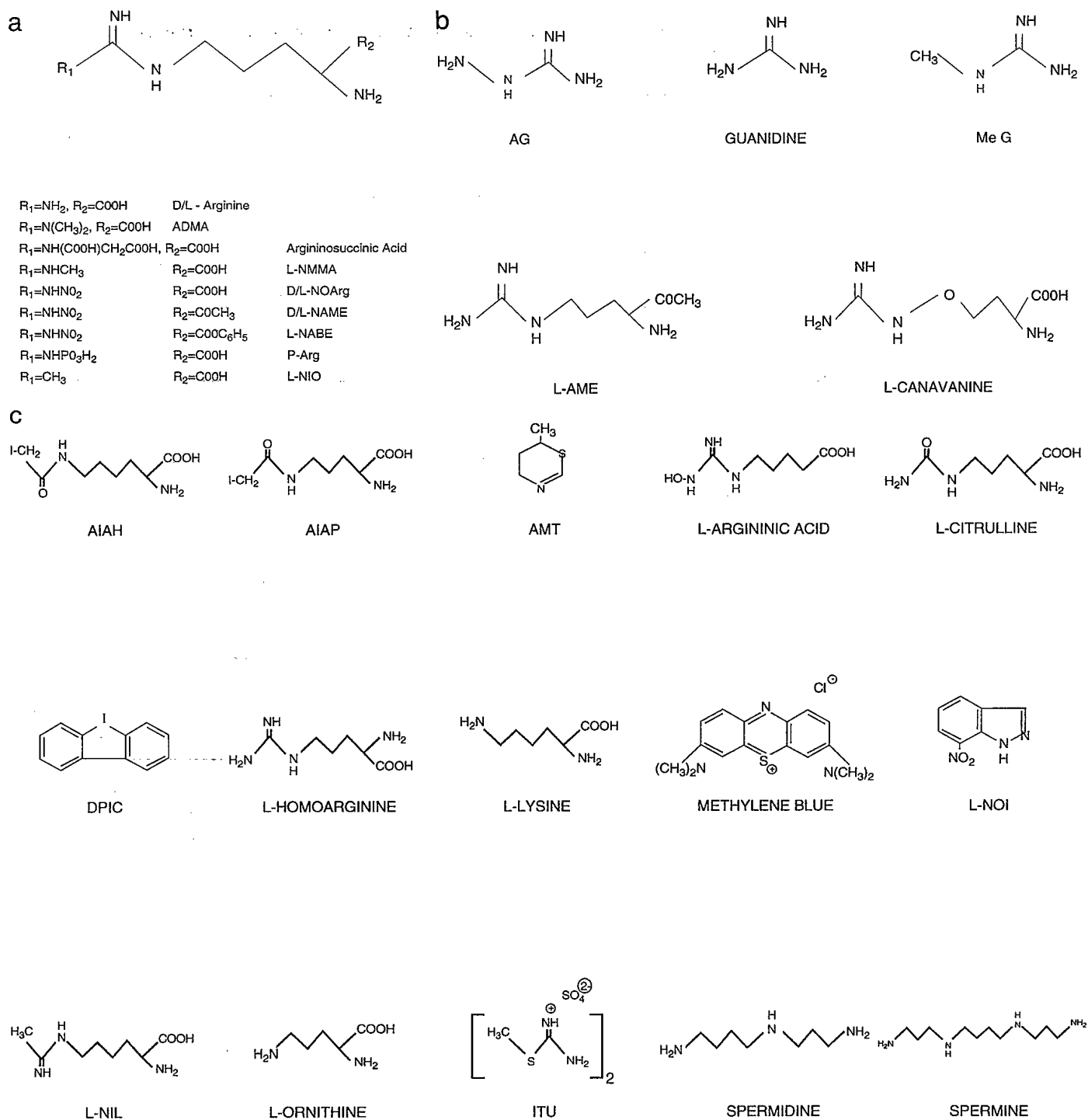
FIG. 2. Structures of test compounds used in this study.
