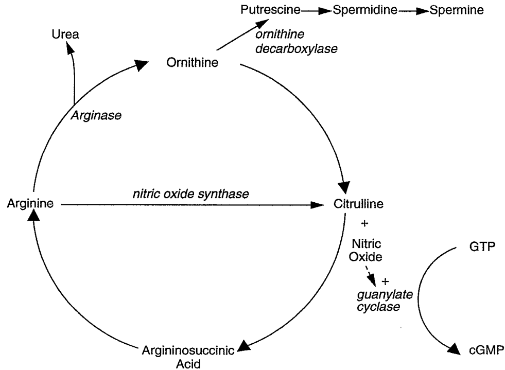
FIG. 1. Biochemical pathways utilizing arginine. Note that nitric oxide activates guanylate cyclase and promotes the conversion of GTP to cGMP.
