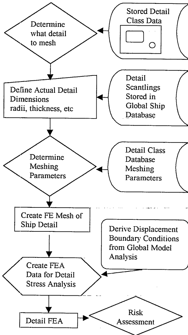
Figure 2: Schematic of top-down analysis with detail class FE mesh data
