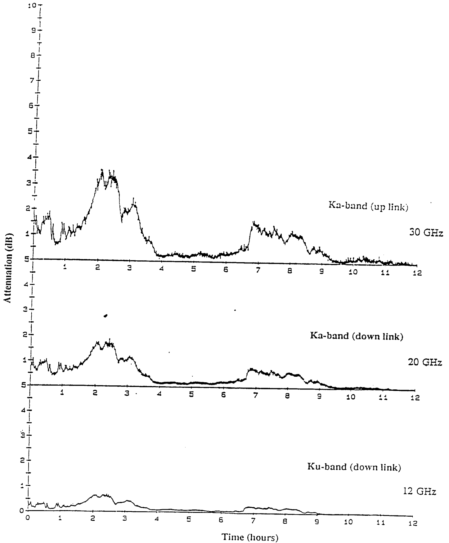
Figure 20: Radiometrically- Measured Path Attenuations, event on Feb 26, 1992.
