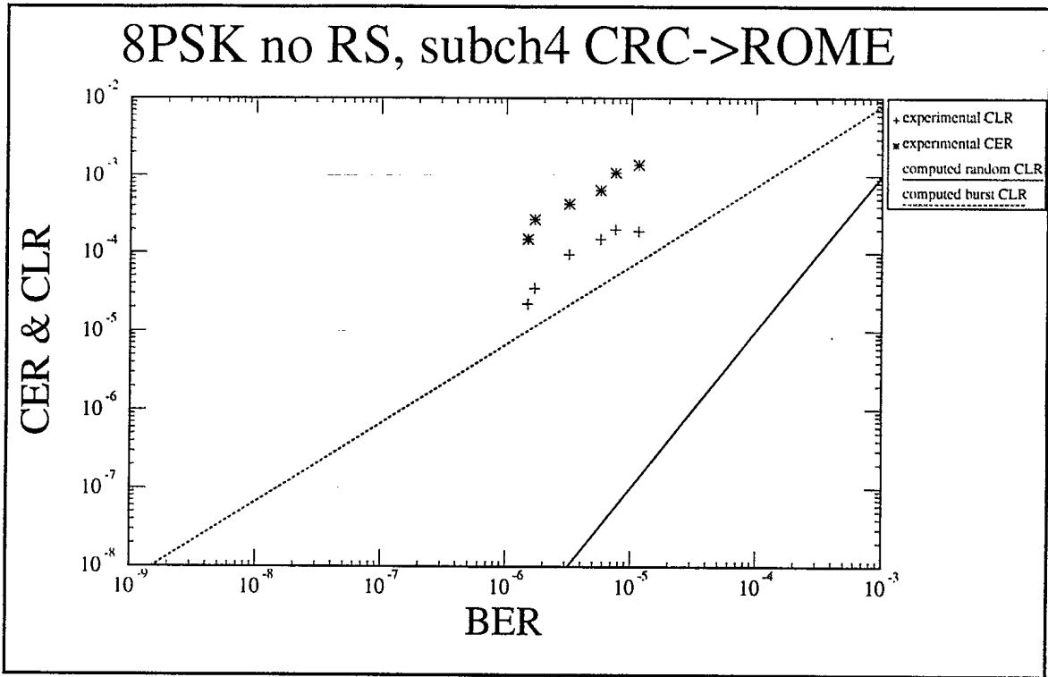
Figure13: 8PSK subchannel 4DS0 CRC->Rome
