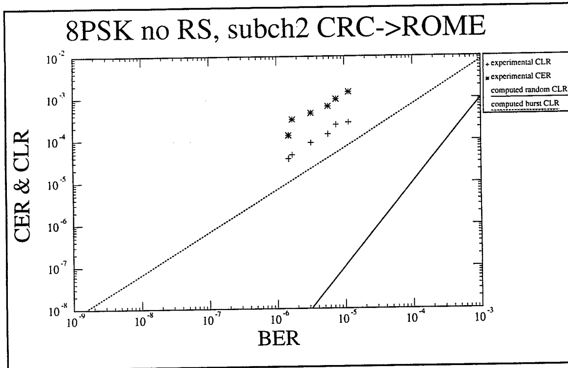
Figure11: 8PSK subchannel DS0 CRC->Rome
