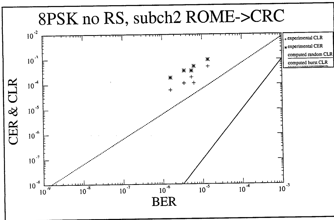
Figure12: 8PSK subchannel DS0 Rome->CRC
