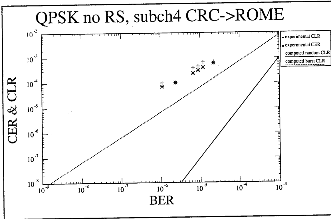
Figure7: QPSK subchannel 4DS0 CRC->Rome
