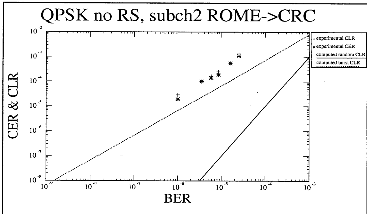
Figure6: QPSK subchannel DS0 Rome->CRC
