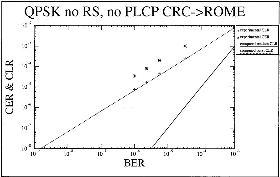
Figure17: QPSK Single channel no PLCP CRC->Rome
