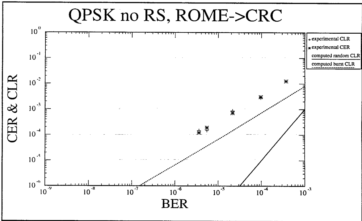
Figure2: QPSK Single channel Rome->CRC
