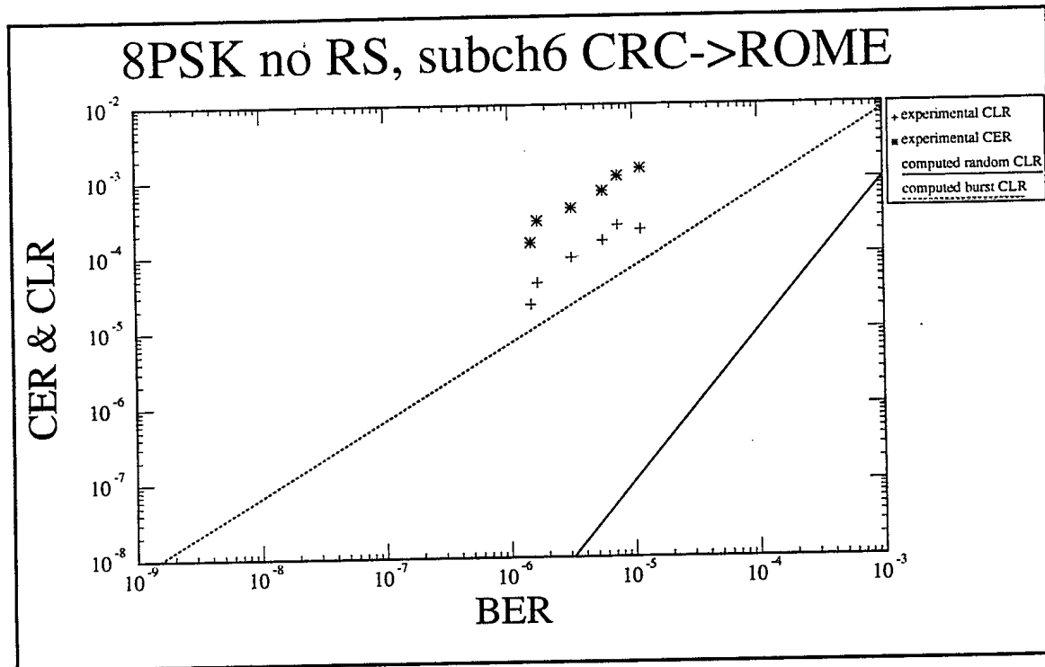
Figure15: 8PSK subchannel DS1 CRC->Rome
