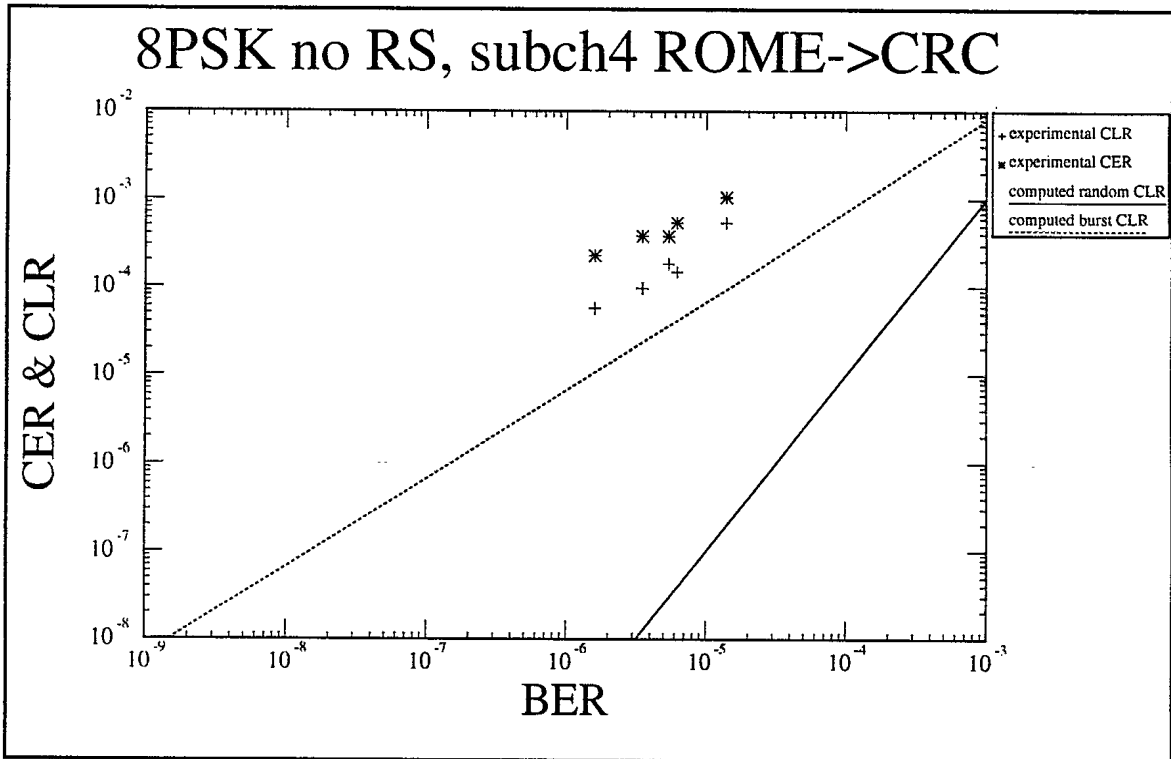
Figure14: 8PSK subchannel 4DS0 Rome->CRC
