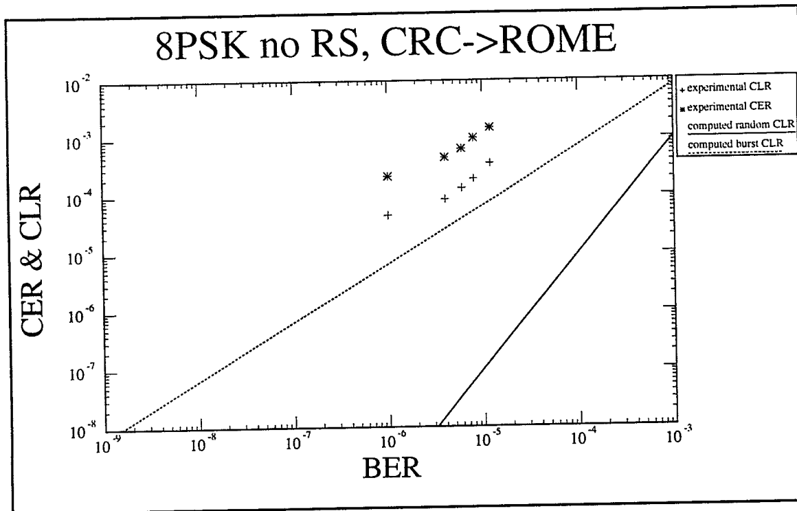
Figure3: 8PSK Single channel CRC->Rome
