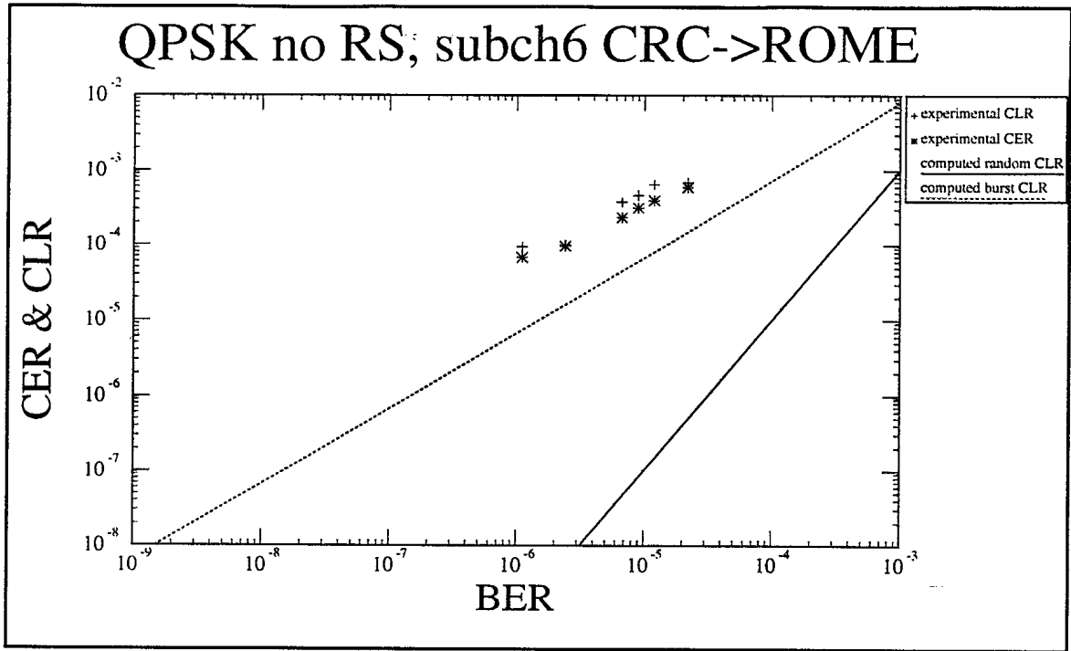
Figure9: QPSK subchannel DS1 CRC->Rome
