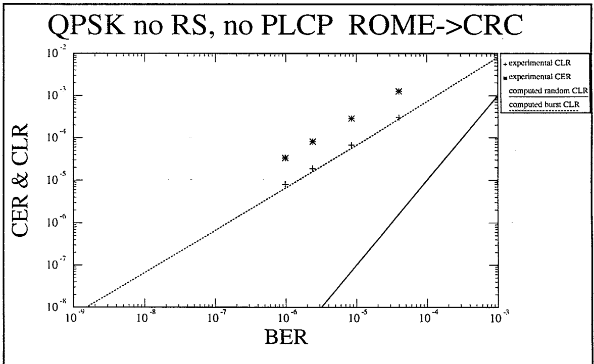
Figure18: QPSK Single channel no PLCP Rome->CRC
