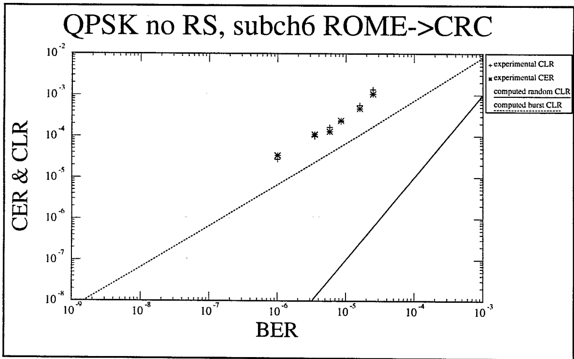
Figure10: QPSK subchannel DS1 Rome->CRC
