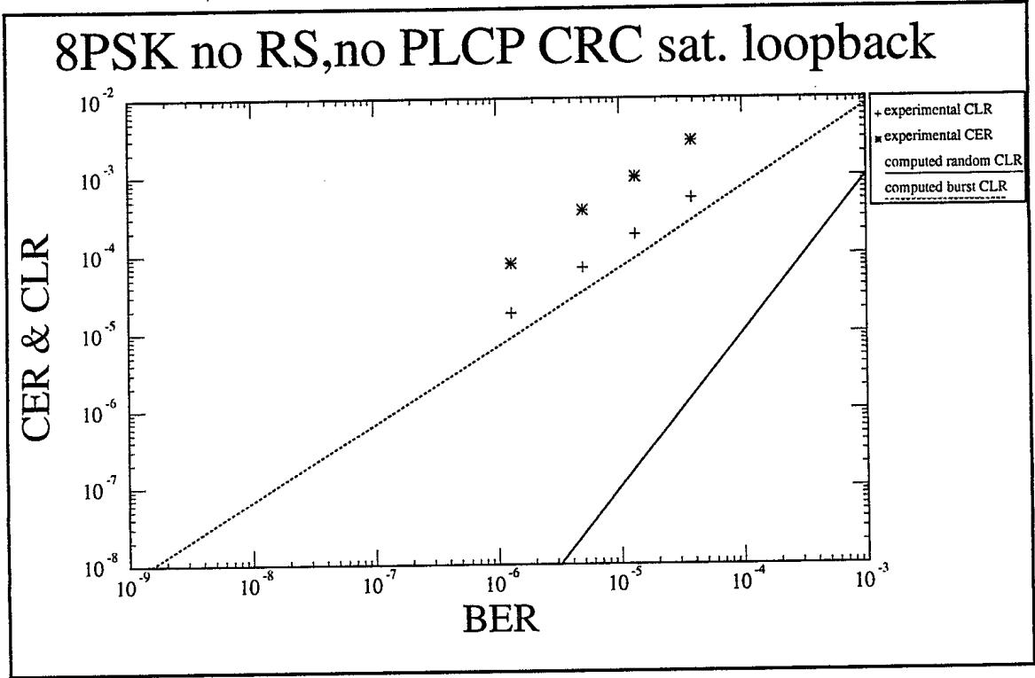
Figure19: 8PSK Single channel no PLCP satellite loopback
