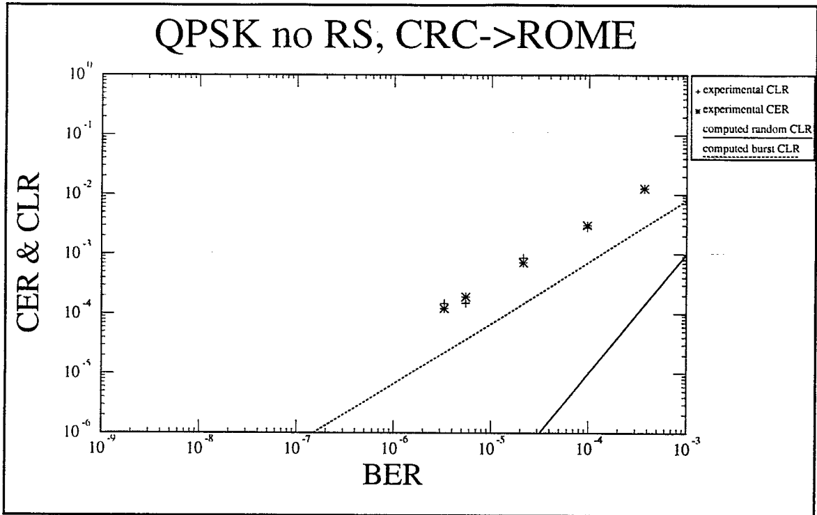
Figure1: QPSK Single channel CRC->Rome
