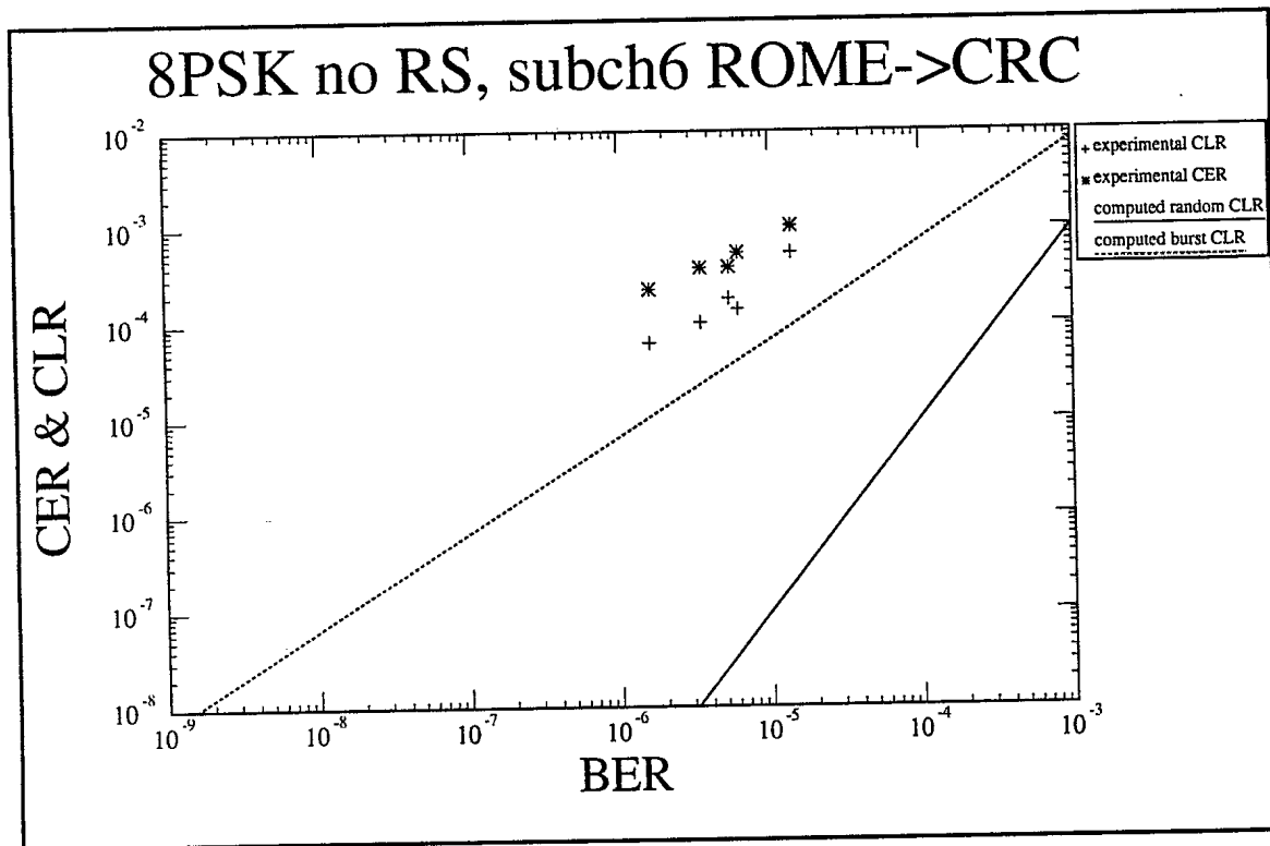
Figure16: 8PSK subchannel DS1 Rome->CRC
