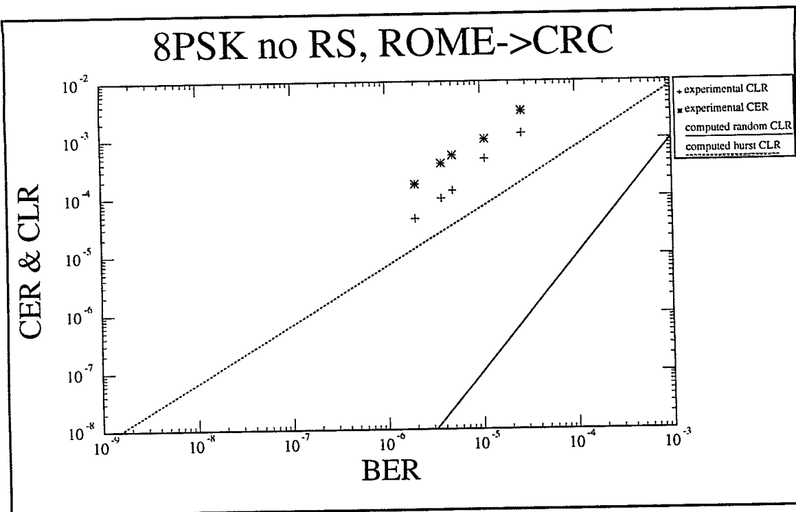
Figure4: 8PSK Single channel Rome->CRC
