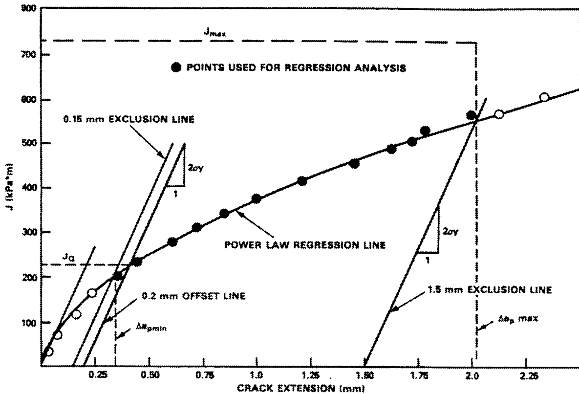
FIGURE 2.: A typical J-crack growth resistance curve [1].
