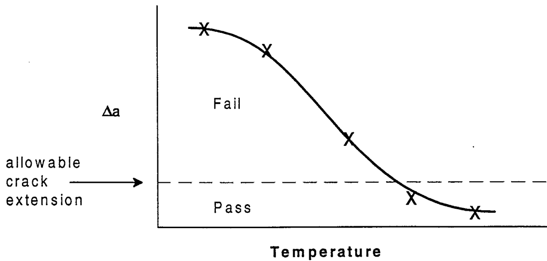
FIGURE 8.: Expected results from proposed test method. Only one specimen is required to produce each data point.
