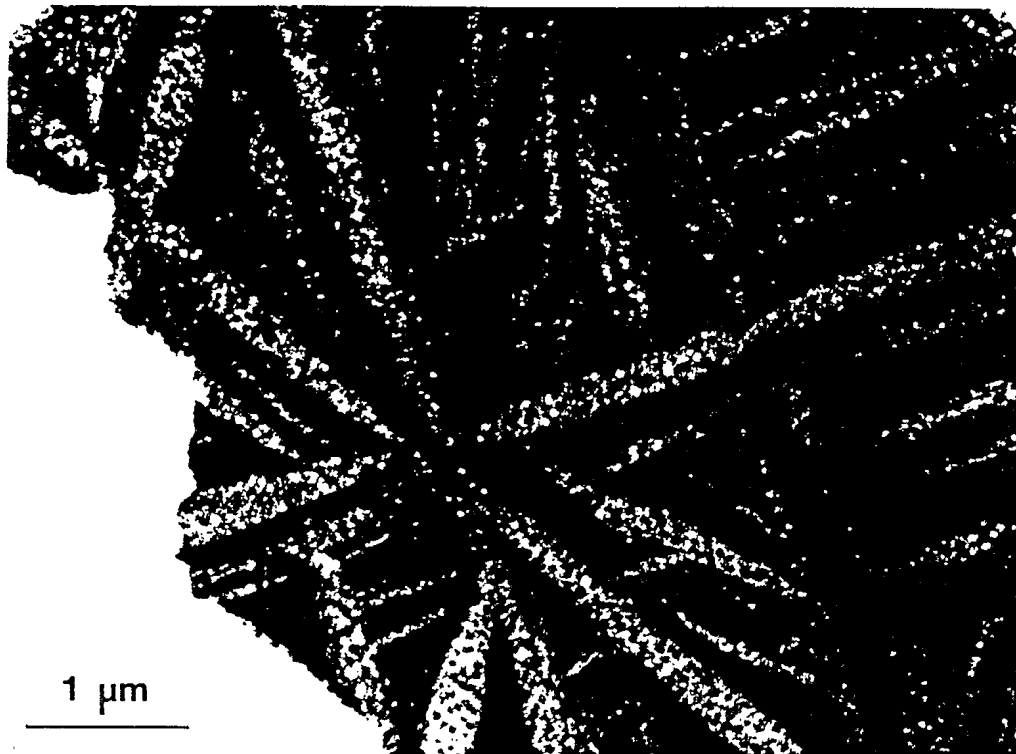
Figure 4: Typical TEM micrograph of the as-deposited region-of a NAB laser cladding showing Widmanstatten \alpha rods (light) and martensite plates (dark).
