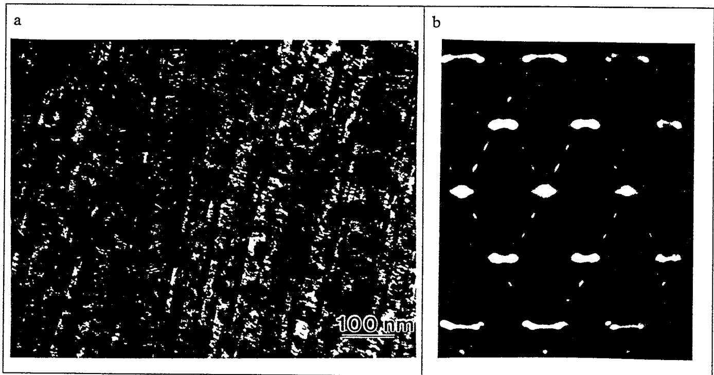
Figure 9: (a) TEM micrograph of martensite in the as-deposited region showing parallel-sided, acicular twins. (b) Corresponding [1\bar{1}20] zone axis SAD pattern for the martensite revealing the presence of 9R order and twinning
