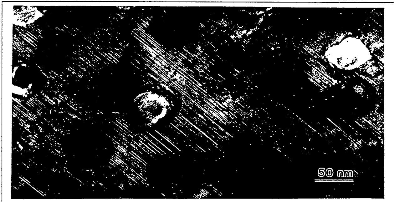
Figure 7: TEM image of an \alpha rod with 9R long-range order. Closely spaced, parallel striations visible in the image are a periodic array of stacking faults on the \{111\}_{fcc} planes..
