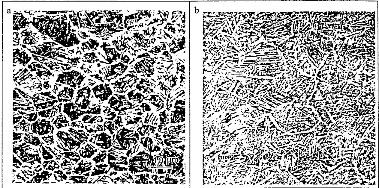
Figure 3: Optical micrographs showing typical microstructures for (a) the as-deposited and (b) reheat zones of a NAB laser cladding.
