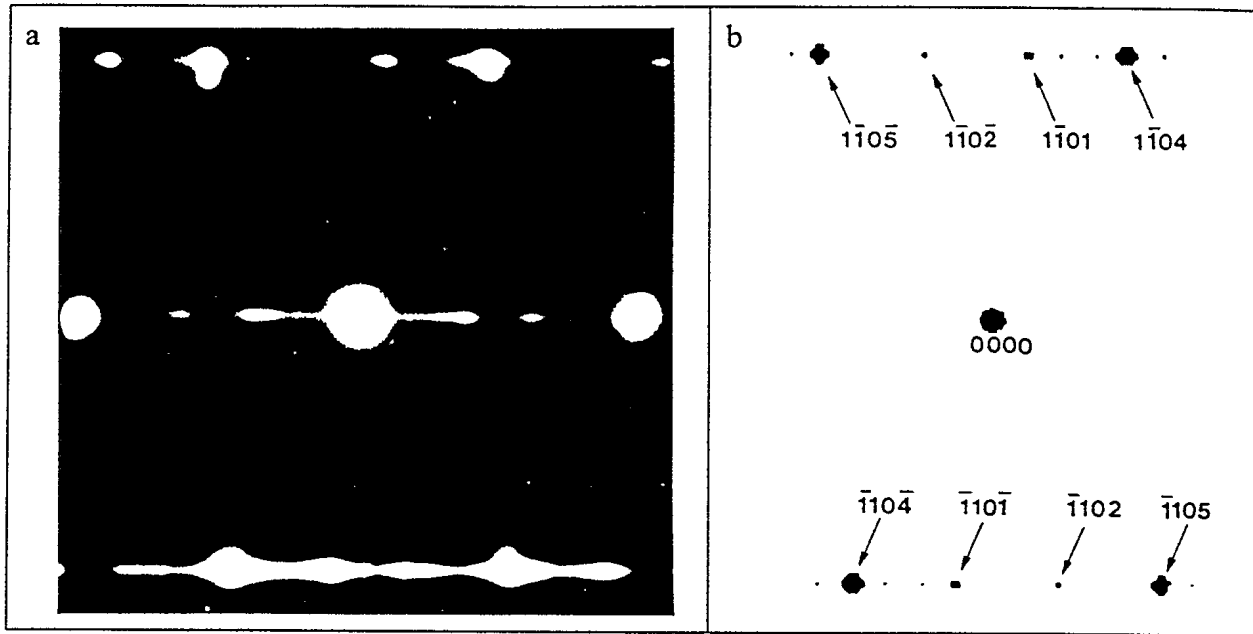
Figure 8: (a) [1\bar{1}20] zone axis SAD pattern for the long-range ordered 9R \alpha phase. (b) Corresponding calculated pattern for a ABCBCACAB stacking module.
