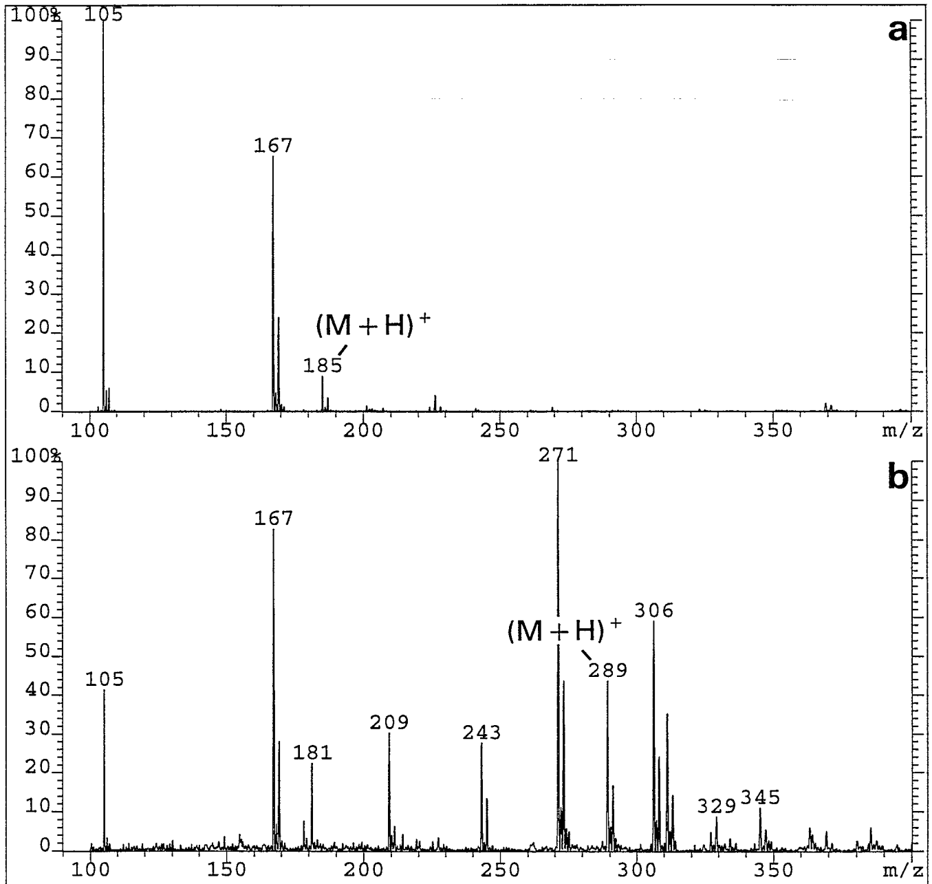
Figure 5: Typical ESI-MS data for a) 8-chloro-6-oxa-3-thia-1-octanol and b) 14-chloro-6,12-dioxa-3,9-dithia-1-tetradecanol obtained during LC-ESI-MS analysis of HT and HQ hydrolysis samples.
