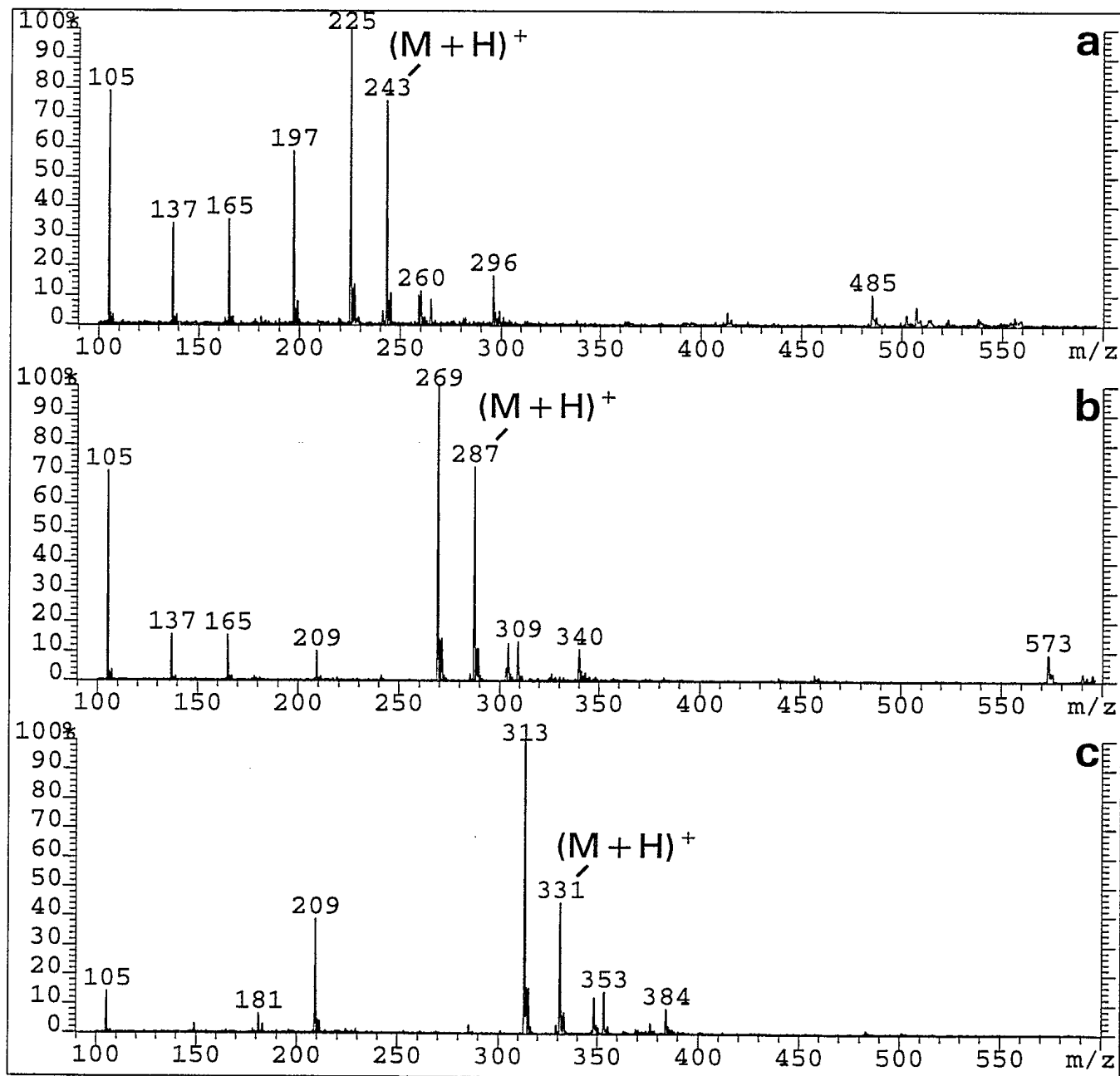
Figure 3: Typical ESI-MS data for a) 3,6,9-trithia-1,11-undecanediol, b) 6-oxa-3,9,12-trithia-1,14-tetradecanediol and c) 6,12-dioxa-3,9,15-trithia-1,17-heptadecanediol (or 6,15-dioxa-3,9,12-trithia-1,17-heptadecanediol) obtained during LC-ESI-MS analysis of HT and HQ hydrolysis samples.
