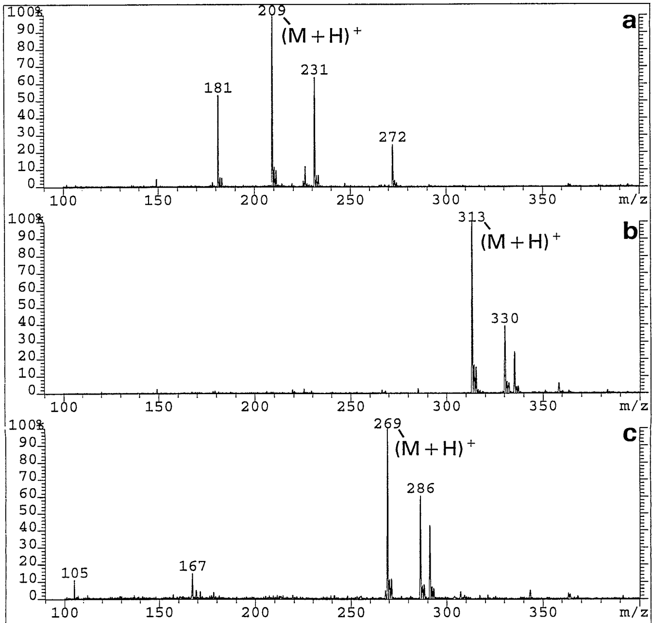
Figure 4: Typical ESI-MS data for a) 1,7-dioxa-4,10-dithiacyclododecane, b) 1,7,13-trioxa-4,10,16-trithiacyclooctadecane (or another isomer) and c) 1,7-dioxa-4,10,13-trithiacyclopentadecane obtained during LC-ESI-MS analysis of HT and HQ hydrolysis samples.
