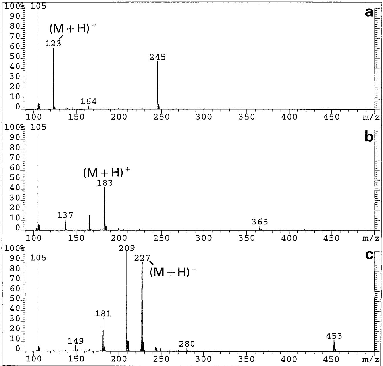
Figure 2: Typical ESI-MS data for a) thiodiglycol, b) 3,6-dithia-1,8-octanediol and c) 6-oxa-3,9-dithia-1,11-undecanediol obtained during LC-ESI-MS analysis of HT and HQ hydrolysis samples.
