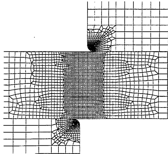
Figure 3: Close up view of shear region in the die-specimen-punch assembly
