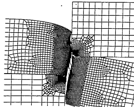
Figure 7b: Predicted crack using MSS criterion with \dot{\gamma}_{crit} = 28.125 \text{ s}^{-1} for Remco iron
