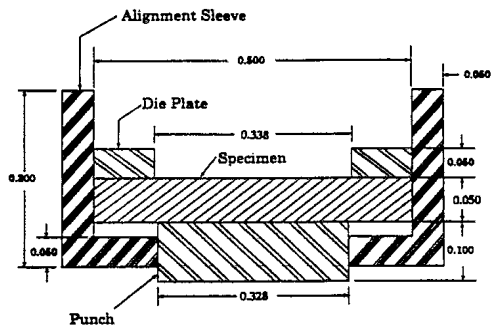
Figure 1: Shear specimen assembly
