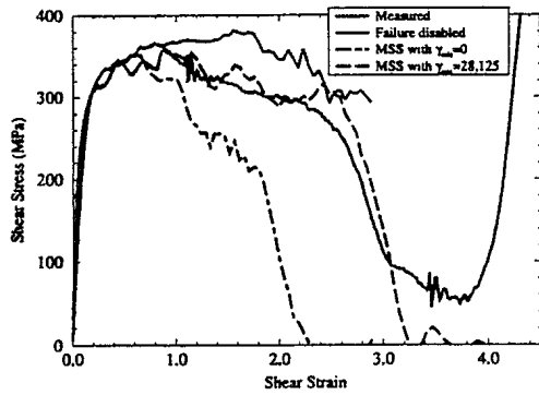
Figure 6: Nominal shear stress-strain curve for numerical model using the MSS criterion and experiment for annealed Remco iron
