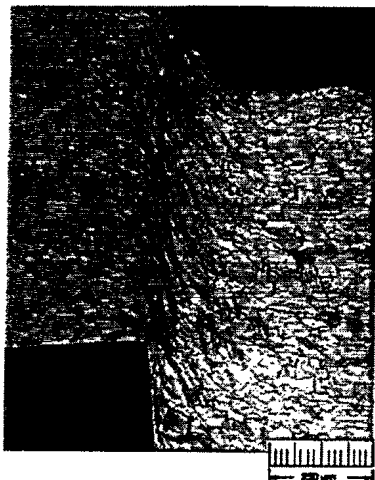
Figure 4: Optical micrograph showing shear region in annealed Remco iron
