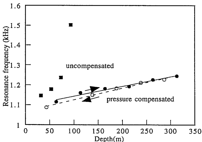
Figure 1 The resonance frequency as a function of depth for a Barrel Stave Projector with and without pressure compensation.
