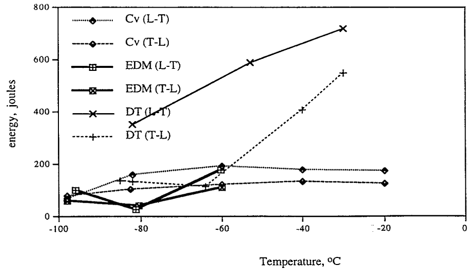
Figure 3: Lower Bound Cv, EDM (Cv) and DT Transition Curves for A517.
