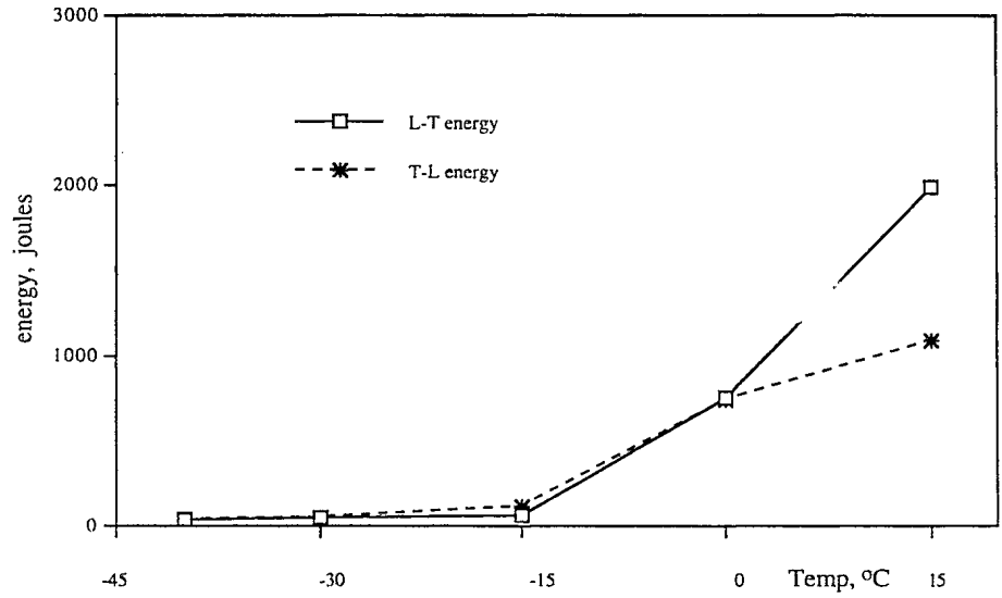
Figure 6a: Dynamic Tear Energy for 15 mm 350WT steel.
