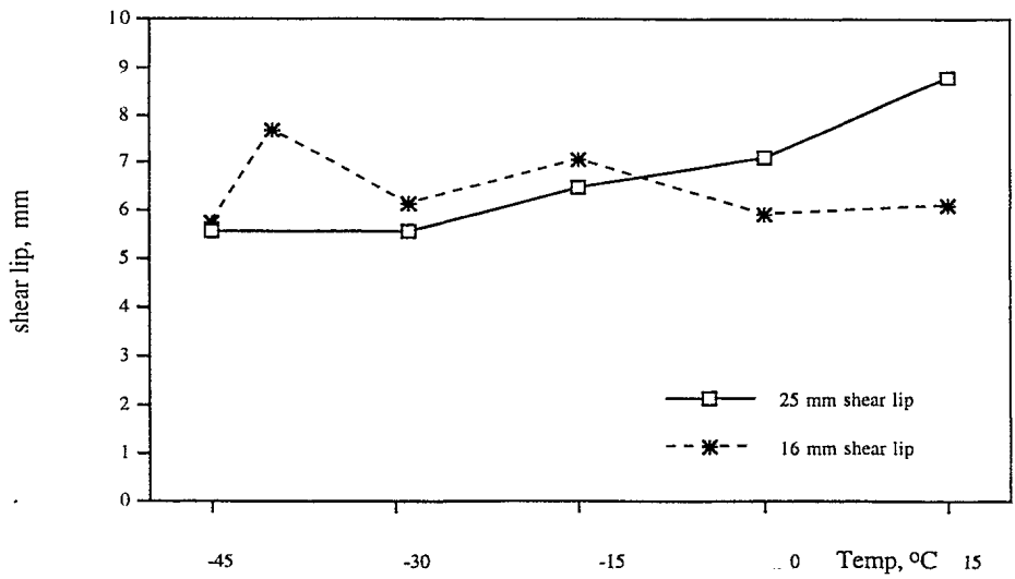
Figure 7b: Shear Lip Results for HY80 GMAW Weld Produced With Standard L-Tec Machine, TIME gas, in the Vertical Position.
