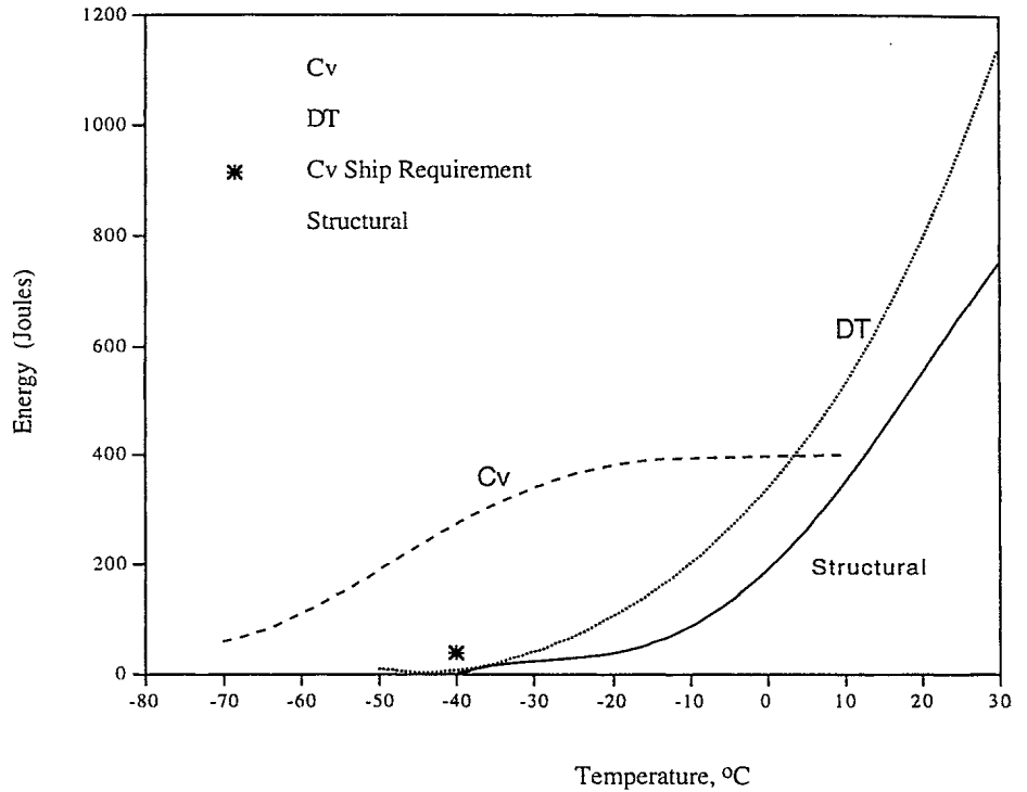
Figure 1: Schematic of Basic Material Design to Guarantee Ductile Behaviour. (In this schematic, the requirement seems reasonable; the material (Cv) seems much better than the requirement; but the structure is unacceptable: this is typical)
