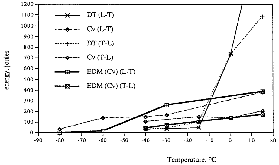
Figure 2: Lower Bound Cv, EDM (Cv) and DT Transition Curves for 350 WT.
