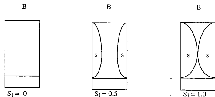
Figure 4: Typical morphologies for dynamic tear impact samples (shear index is measured at the point of the closest contact between the two shear lips: S_I = 2s/B ).
