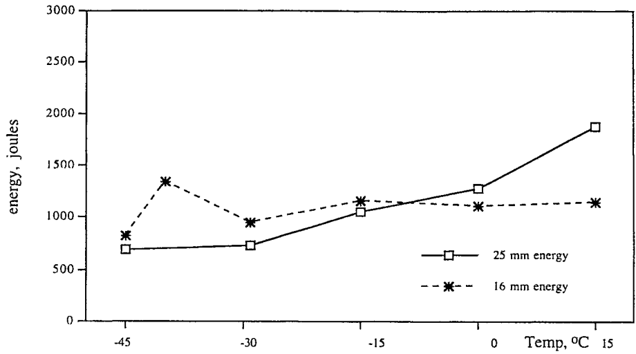
Figure 7a: Dynamic Tear Energy for HY80 GMAW Weld Produced With Standard L-Tec Machine, TIME gas, in the Vertical Position.
