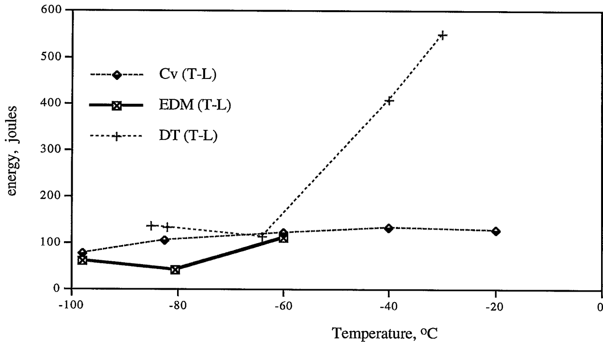
Figure 3c: Lower Bound Cv, EDM (Cv) and DT Transition Curves for A517 (T-L).
