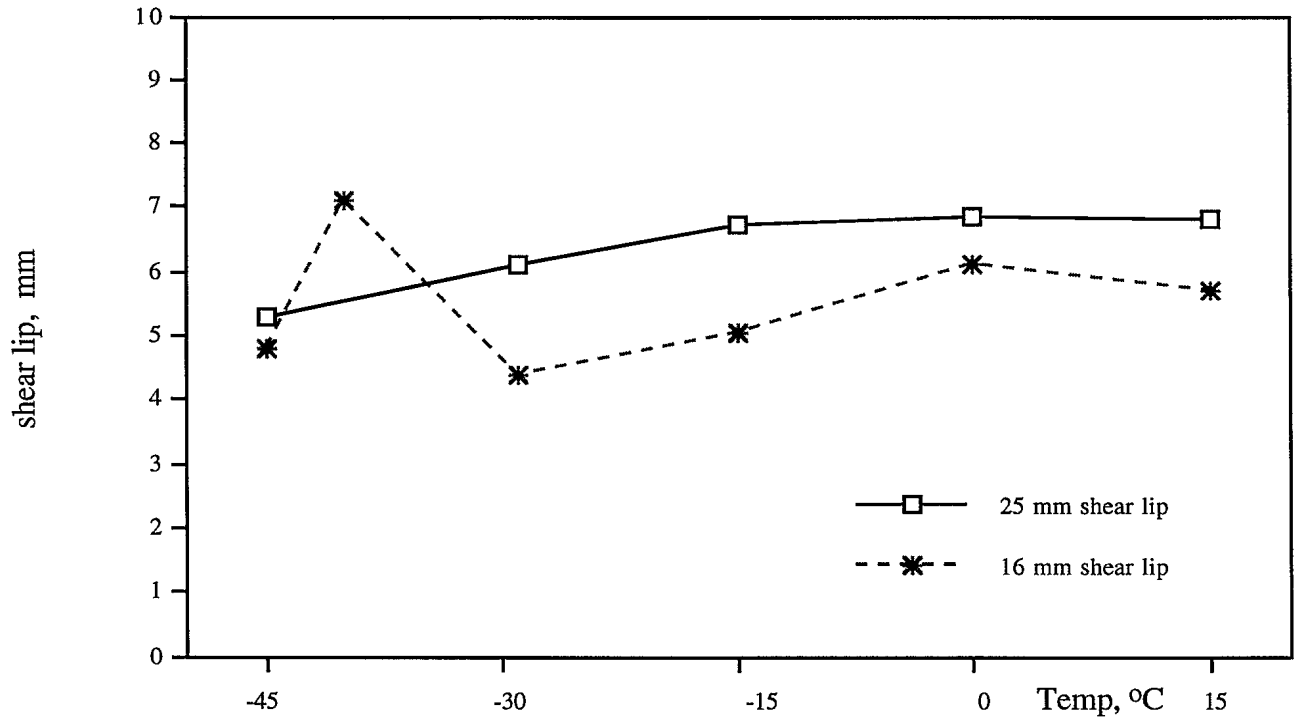
Figure 10b: Shear Lip Results for HY100 GMAW Weld Produced With Pulsed Fronius Machine, 95/5 gas, in the Overhead Position.
