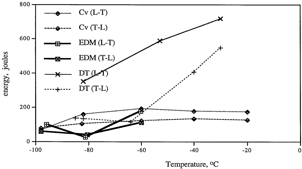
Figure 3b: Lower Bound Cv, EDM (Cv) and DT Transition Curves for A517.
