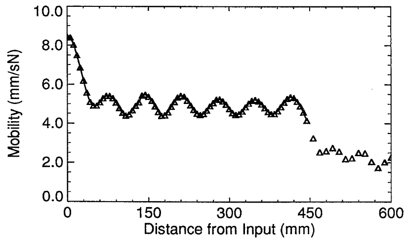
Figure 4: Beam with 3/8" Damping
