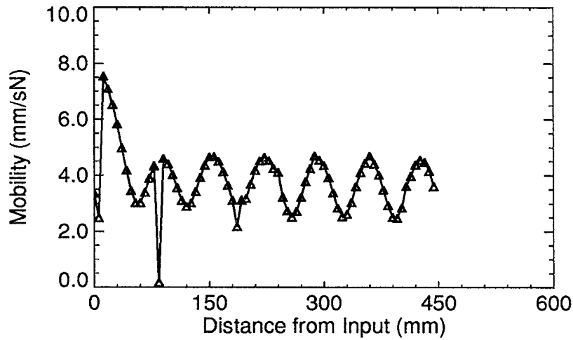
Figure 3: Beam with 1/4" Damping
