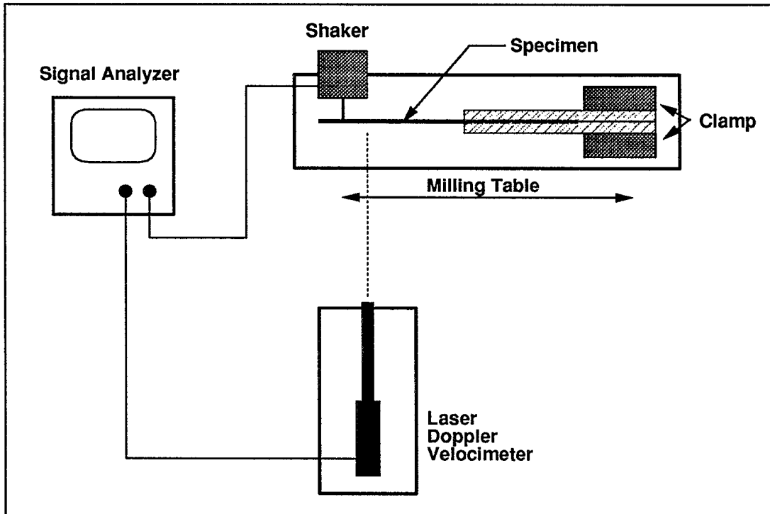
Figure 2: Schematic of Test Setup
