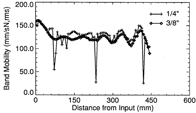
Figure 10: Combined RMS Tests - Mobility
