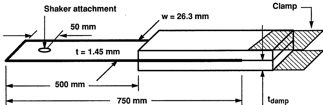
Figure 1: Sketch of Test Sample
