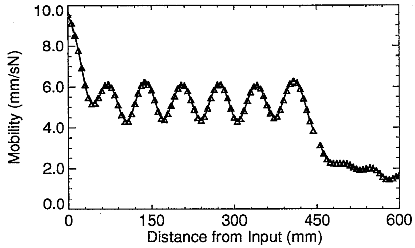
Figure 5: Beam with 1/2" Damping
