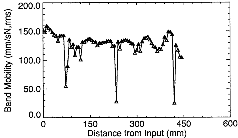
Figure 8: Beam with 1/4" Damping
