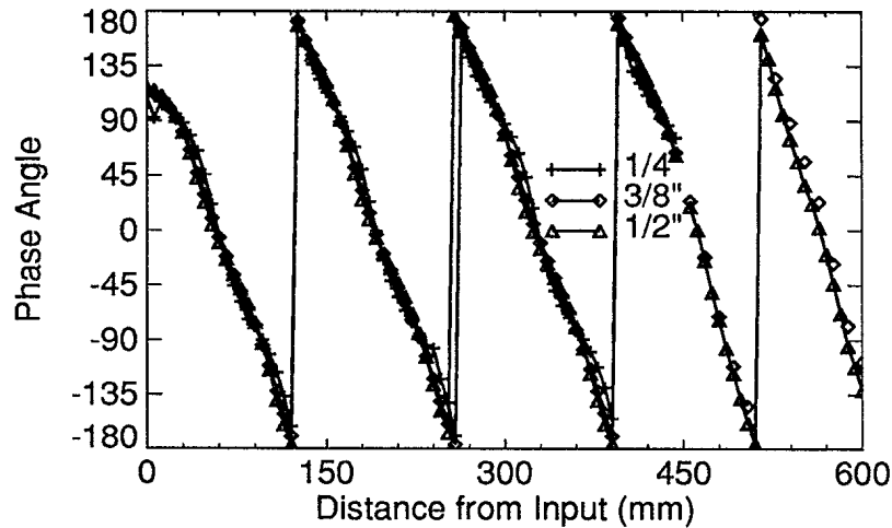
Figure 7: Combined Pure Sine Tests - Phase
