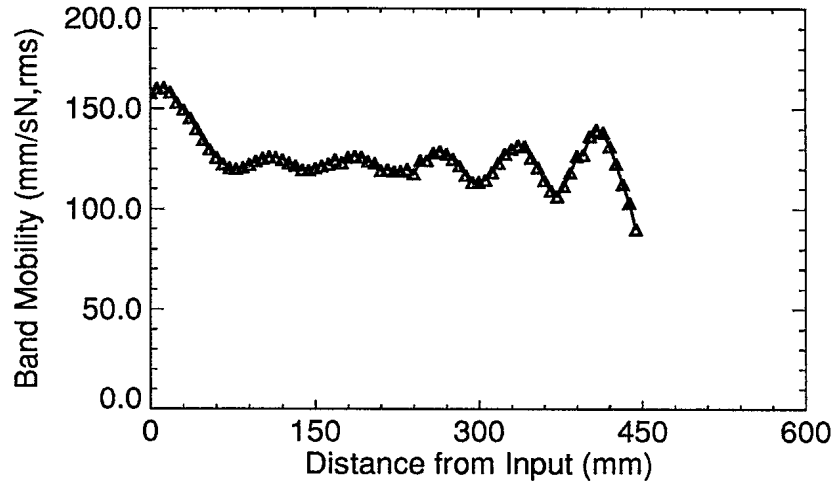
Figure 9: Beam with 3/8" Damping
