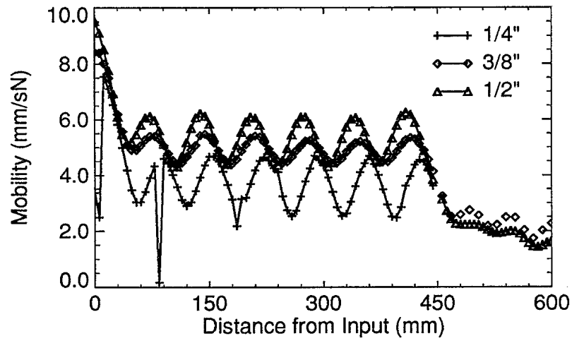
Figure 6: Combined Pure Sine Tests - Mobility
