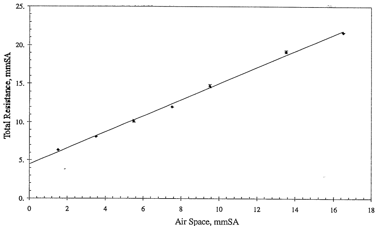
Figure 1. Calibration results of the water vapour permeability apparatus. Total Resistance is the measured water vapour resistance of the Air Space (between the wet and dry surfaces) and the intrinsic apparatus resistance. Error bars represent one standard deviation from the mean but the standard deviation is generally small and the error bars are often obscured by the data point marker.
