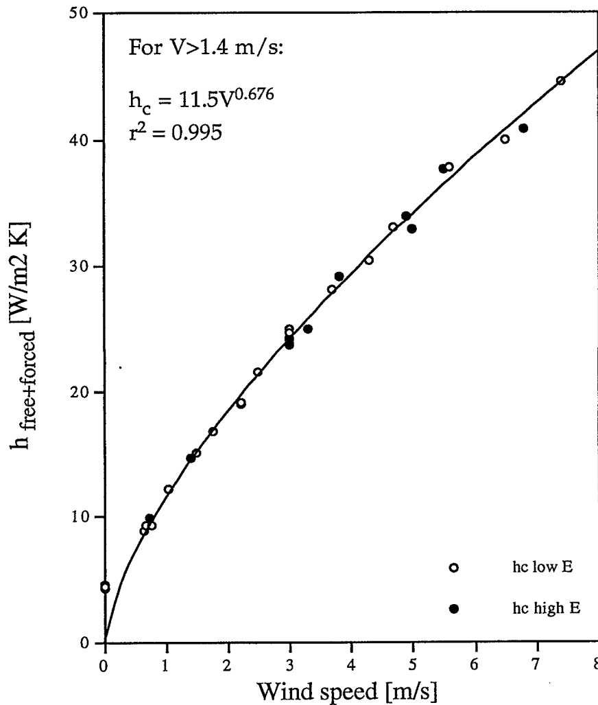
Figure 2. Convective heat transfer coefficients for the three-zone head with high and low emissivity surfaces.
