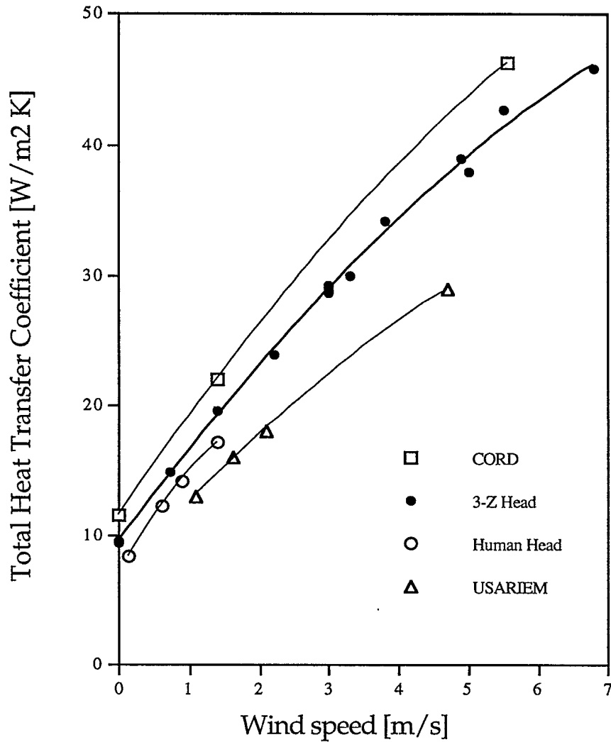
Figure 3. Heat transfer from the three-zone thermal manikin head compared to values obtained from the heads of two other thermal manikins and from human subjects.
