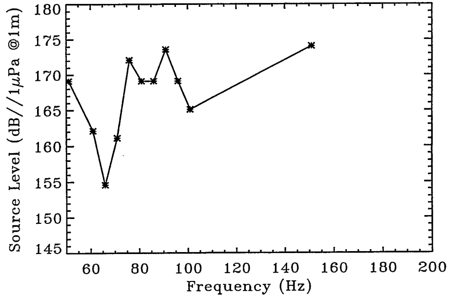
Figure 5. The projector response for a constant driving voltage of 140 V rms with the Argotec head.
