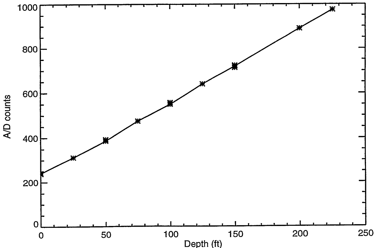
Figure 3. Projector depth sensor calibration.
