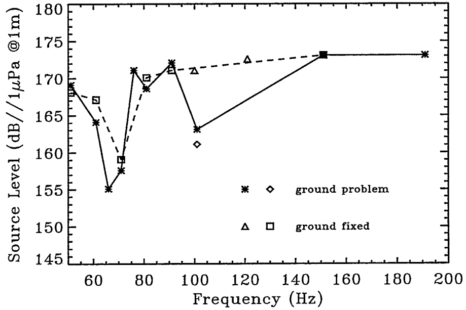
Figure 4. The projector response for a constant driving current of 0.5 A rms with the Argotec head.
