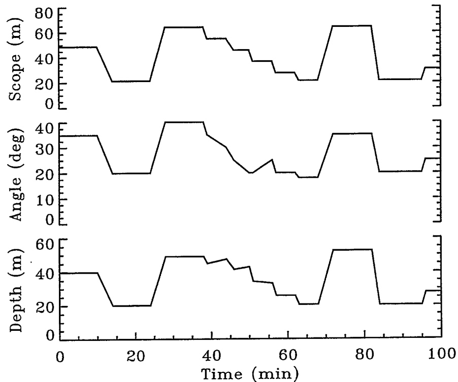
Figure 9. Observed projector towing characteristics at a nominal speed of 3.5 knots.
