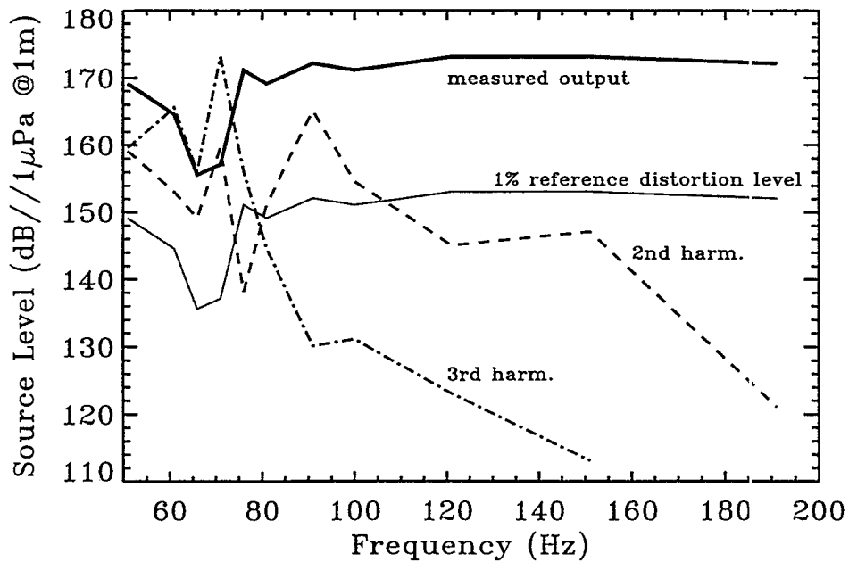
Figure 7. Second and third harmonic levels as a function of frequency. The heavy solid line indicates the measured fundamental level, while the light solid line 20 dB below the drive signal represents a 1% total harmonic distortion reference level.
