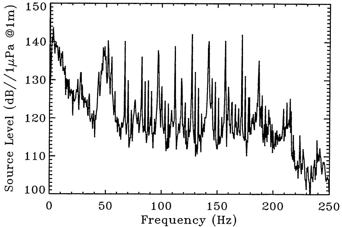
Figure 8. Response of the Argotec 219 projector to the broadband signal JOER.WAV.
