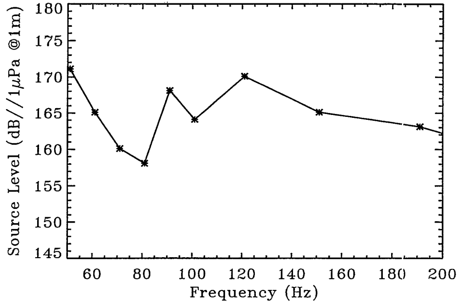
Figure 6. The projector response for a constant driving current of 0.5 A rms with the MRI head.
