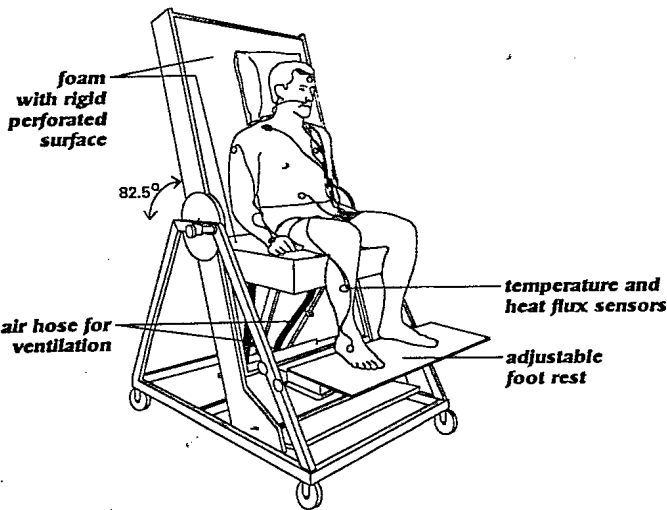
Fig. 1 Schematic of the tilt-table shown in its sitting configuration
