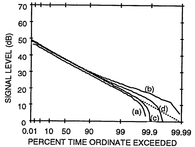
FIGURE 7. Cumulative distributions of data recorded during December 1992 for periods of one hour, (a) slow fading, (b) fast fading; and periods of several days (c) slow fading, (d) fast fading
