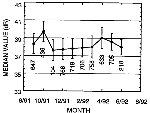
FIGURE 9. Monthly median values of the cumulative distributions of hourly median signal levels. The error bars indicate one standard deviation and each number, the available number of hour medians
