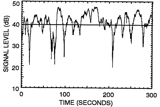
FIGURE 5. Example showing typical received signal level variations during a period of slow fading
