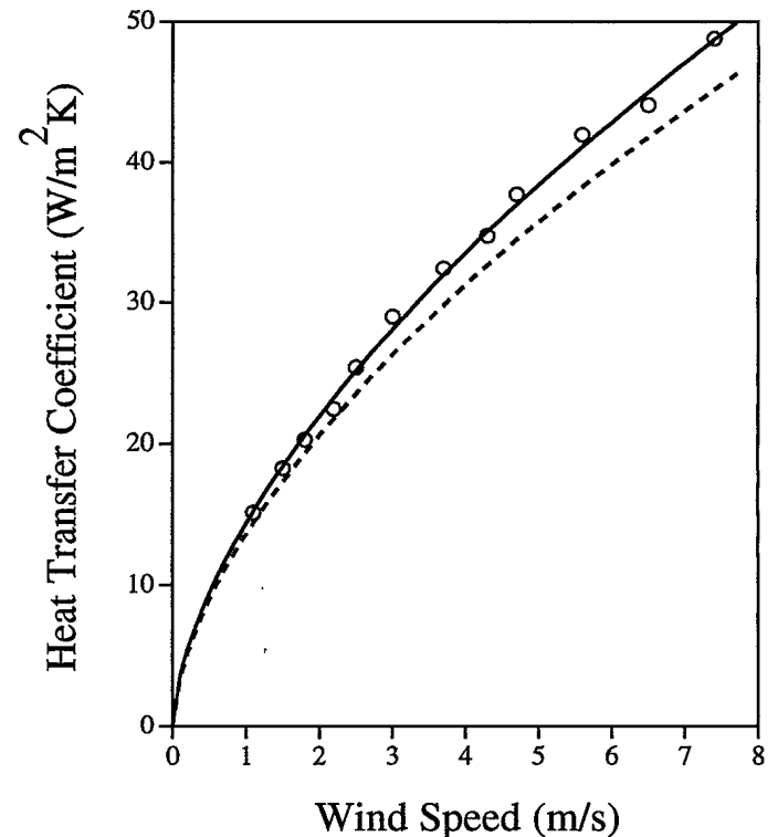
FIG. 1. The experimental values of the convective heat transfer coefficient of the face segment of the thermal simulator are plotted as a function of wind speed. The solid line is the best-fit curve, given by equation 5. The dashed line was calculated for a cylinder of the same diameter as that used by Siple and Passel for their cooling experiment in Antarctica.
