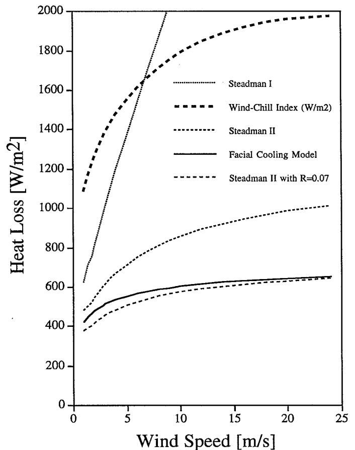
FIG. 7. Comparison of models of the effect of wind on the heat lost from bare skin.
