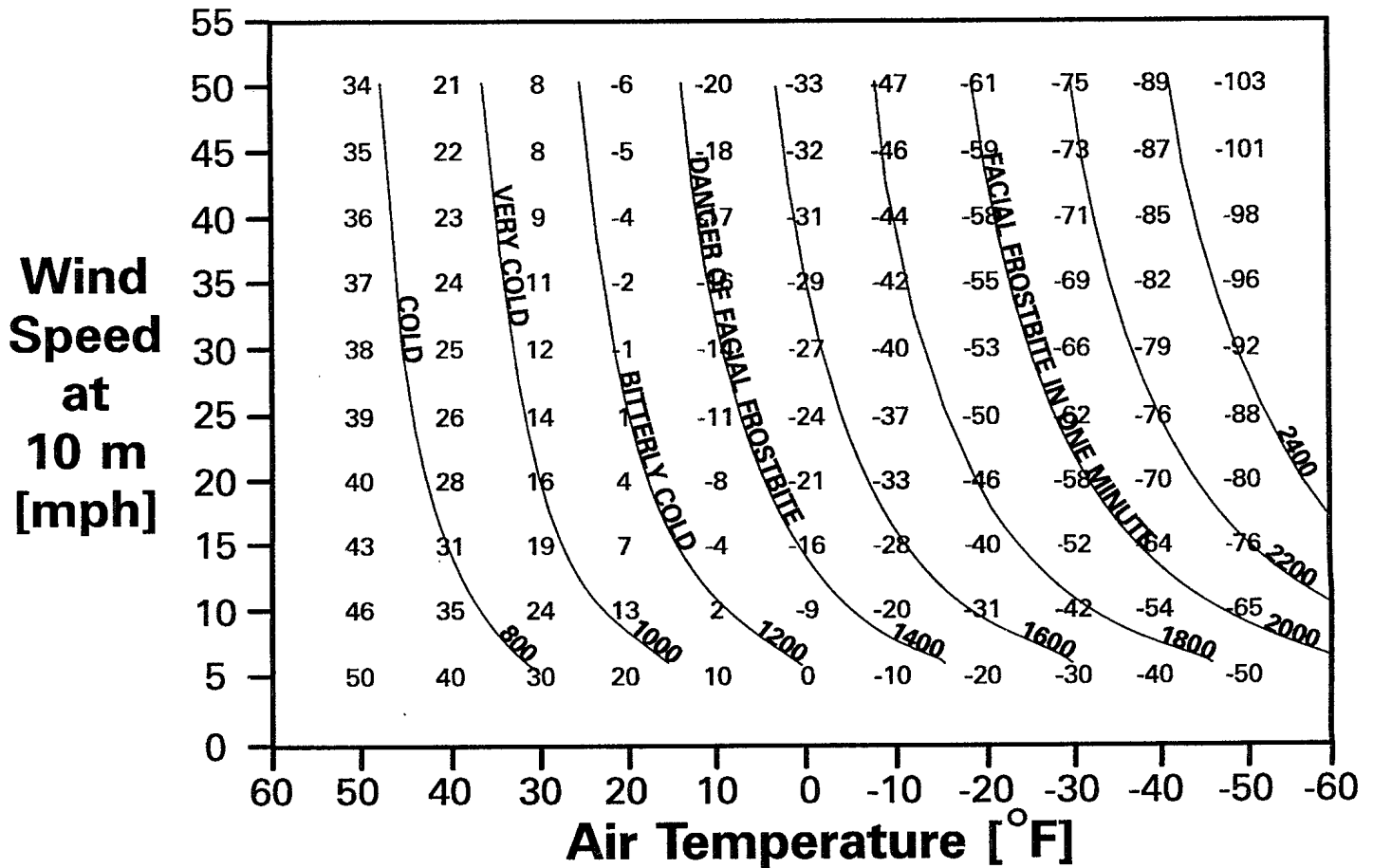
FIG. 6. Wind chill equivalent temperatures in °F, calculated at face level, using the facial cooling model. The curves are lines of constant wind chill index, which are also isotherms of equivalent temperature. Values of the index are noted on the tail of each curve, using the original notation, without units. Wind speeds are those measured at the standard height of 10 m. Increase wind speeds measured at face level by 50% before using the table. In bright sunshine, add 10°F to the equivalent temperature.
