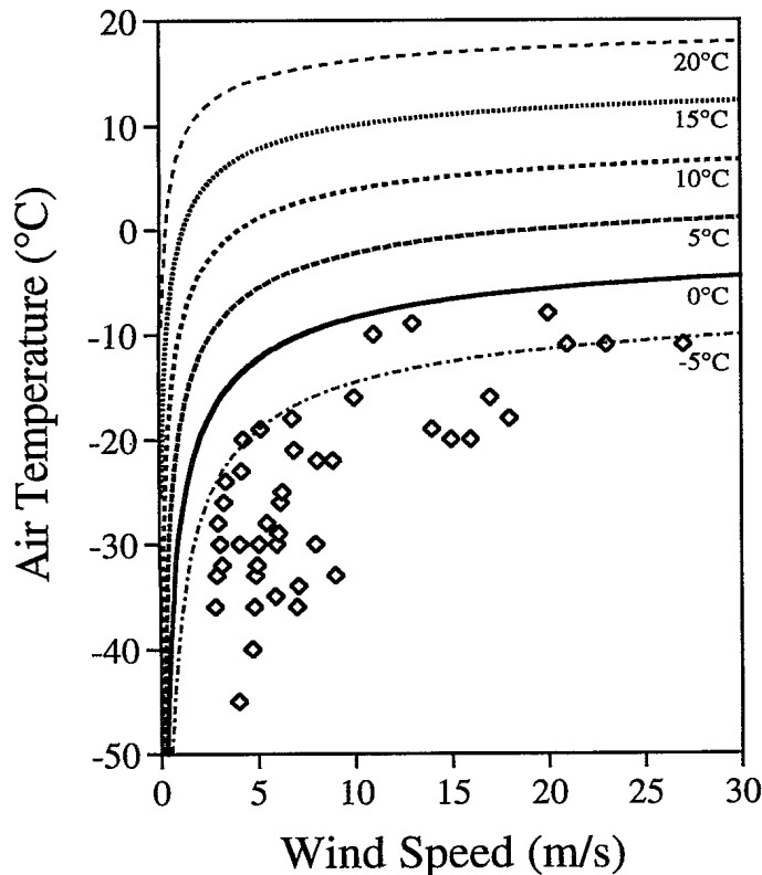
FIG. 3. Skin temperatures calculated from the facial cooling model. The scattered points represent conditions at which frostbite (◊) was reported by Wilson (1964) in the Antarctic.
