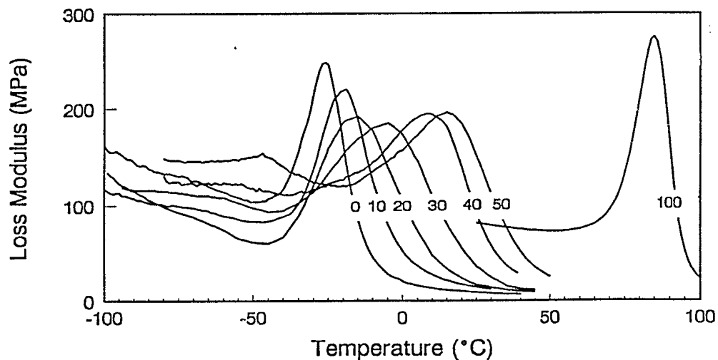
Figure 2. Tensile loss modulus ( E'' ) versus temperature for TPU/PVC samples excited in flex mode at 1 Hz. The number on each curve corresponds to the volume concentration of PVC in percent.
