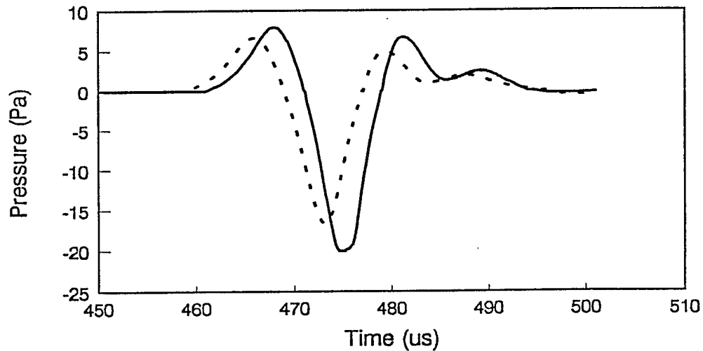
Figure 6. Insertion loss time domain data for reference (—) and 10% PVC blend sample (-----) signals. The polymer sample was 24.4 mm thick.
