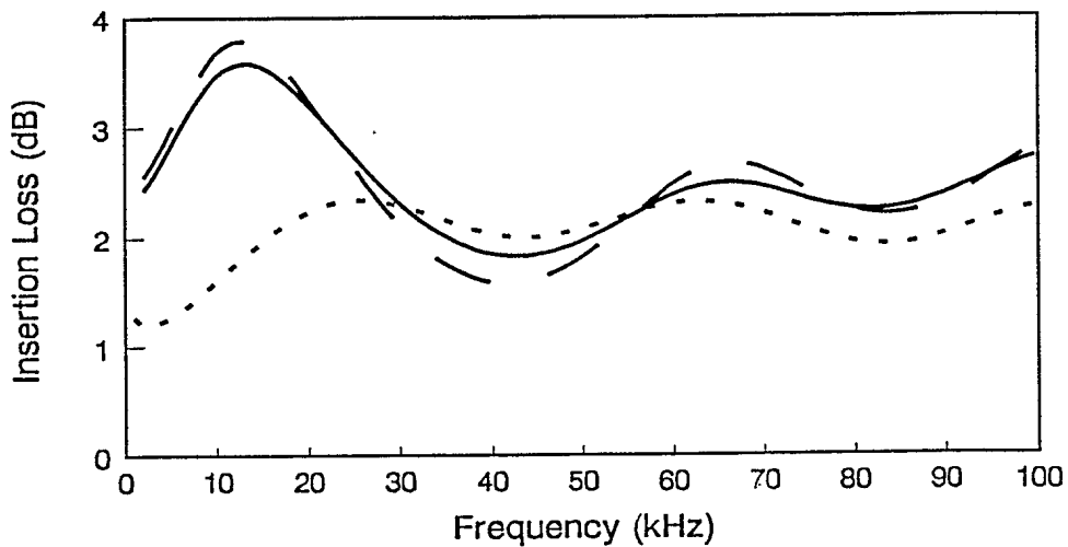
Figure 9. Insertion loss spectra for multilayered sample. The experiment was carried out with the 0% PVC side facing the projector (—) and with the 60% PVC side facing the projector (-----). The simulation (-----) was carried out assuming values of c and \alpha shown in Table I.
