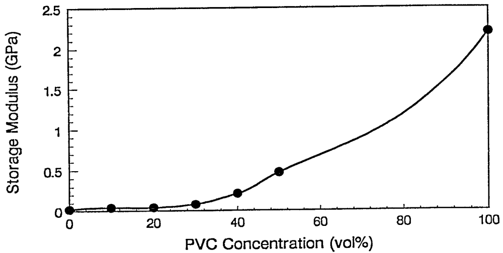
Figure 3. Tensile storage modulus ( E' ) versus PVC concentration for TPU/PVC blends at 23°C and 103 Hz. The solid line is a cubic spline fit (—) to the data points ( \bullet ).
