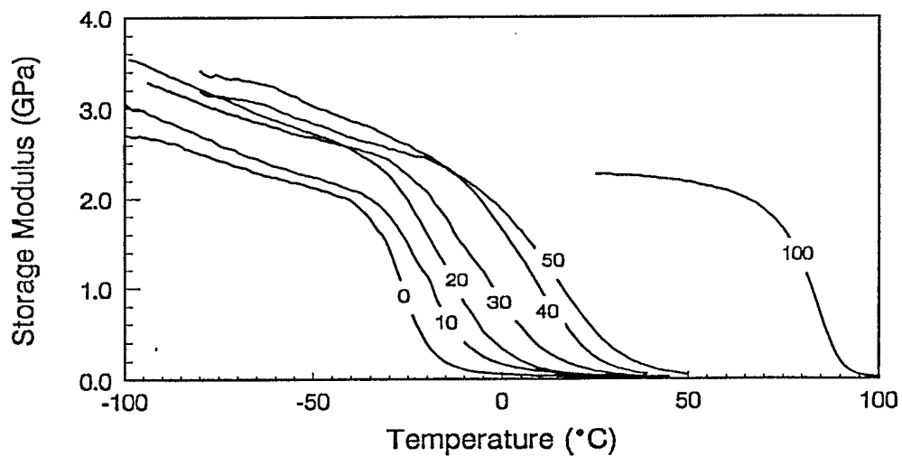
Figure 1. Tensile storage modulus ( E' ) versus temperature for TPU/PVC samples excited in flex mode at 1 Hz. The number on each curve corresponds to the volume concentration of PVC in percent.
