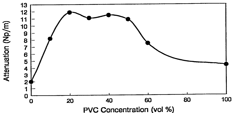
Figure 10. Attenuation coefficients obtained by curve fitting versus PVC concentration for TPU/PVC blends. Data points (●), cubic spline fit (—).
