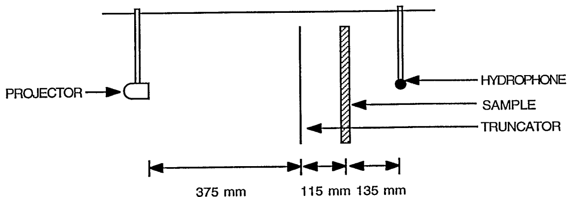
Figure 5. Schematic diagram of insertion loss experiment illustrating relative positions of parametric array projector, truncating plate (acoustic filter), sample, and hydrophone.
