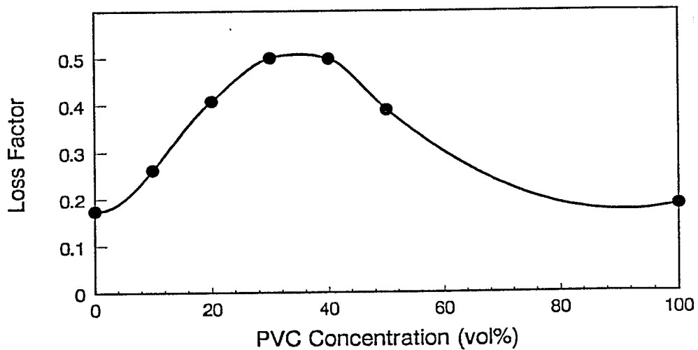
Figure 4. Material loss factor ( \tan \delta ) versus PVC concentration for TPU/PVC blends excited in tension at 23°C and 103 Hz. Data points ( \bullet ), cubic spline fit (—).
