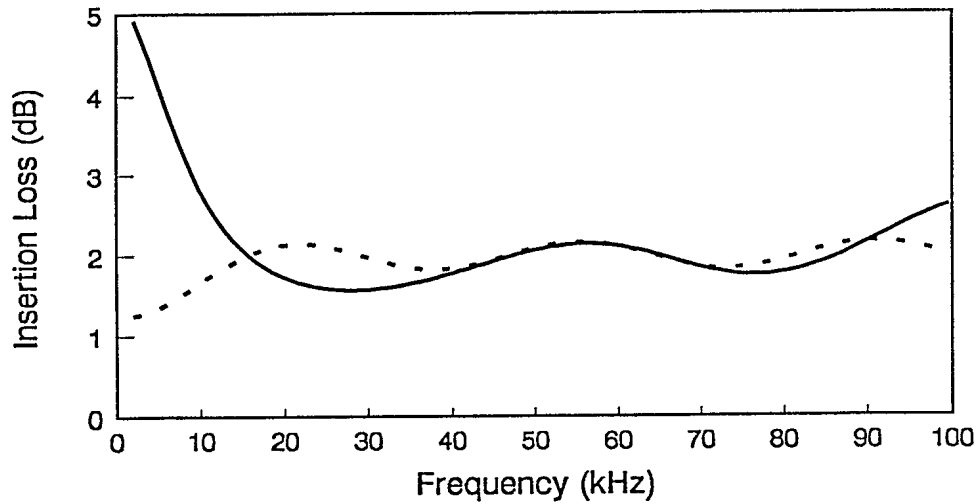
Figure 8. Insertion loss spectra for 10% PVC blend determined by experiment (—) and simulation (-----) using c = 1756 m/s and \alpha = 8.2 Np/m.
