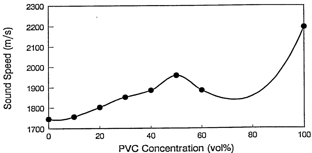
Figure 7. Sound speed calculated from equation (1) versus PVC concentration for TPU/PVC blends. Data points ( \bullet ), cubic spline fit (—).
