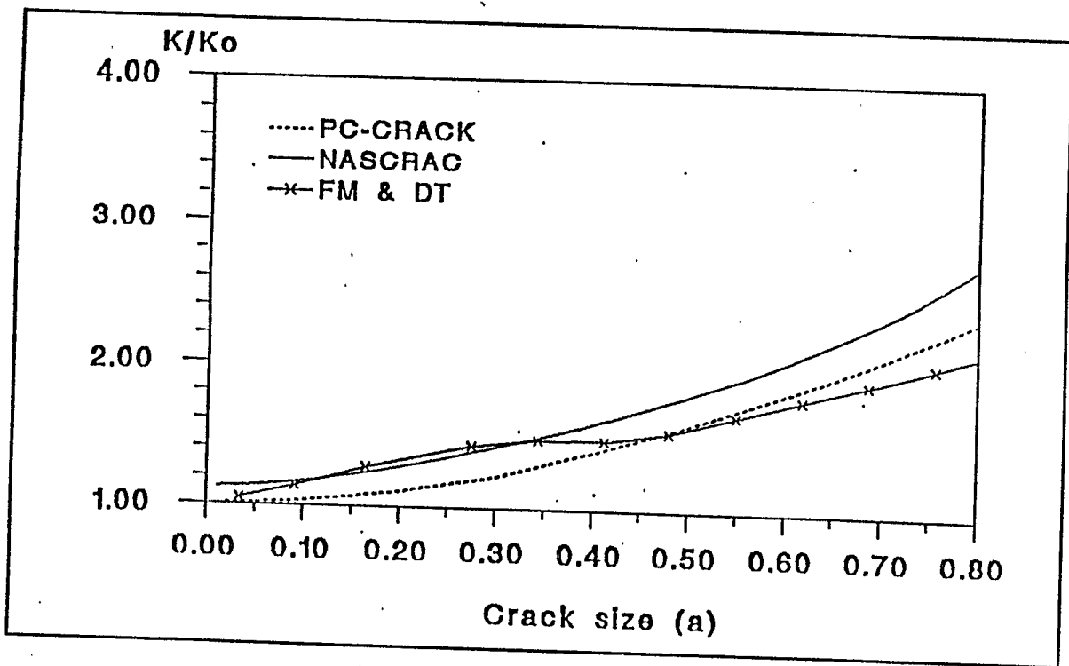
Figure 11. Comparison of K results for cylinder problem
