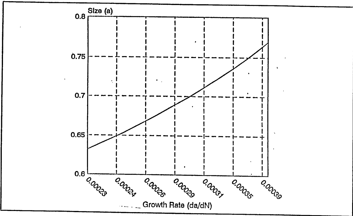
Figure 1. Crack Length vs Growth Rate for pc-CRACK
