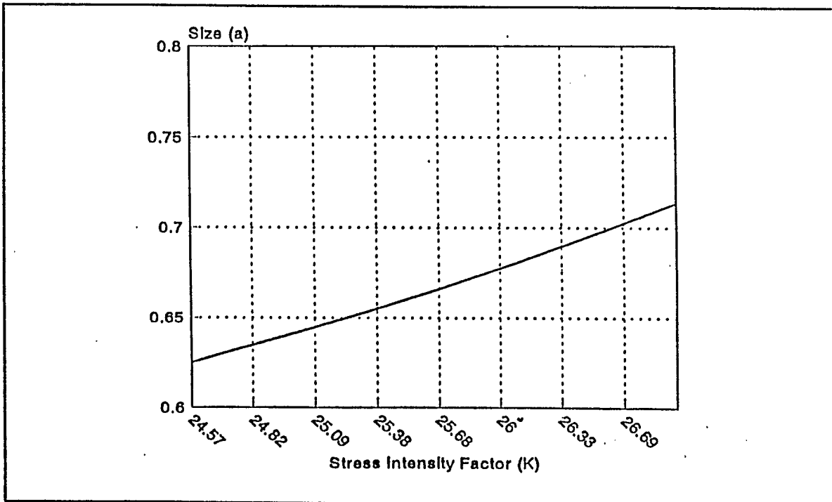
Figure 4. Crack Length vs K for NASCRAC
