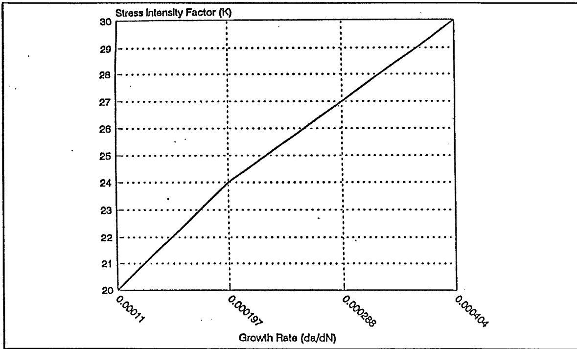
Figure 7. K vs Growth Rate for F.M. & D.T.
