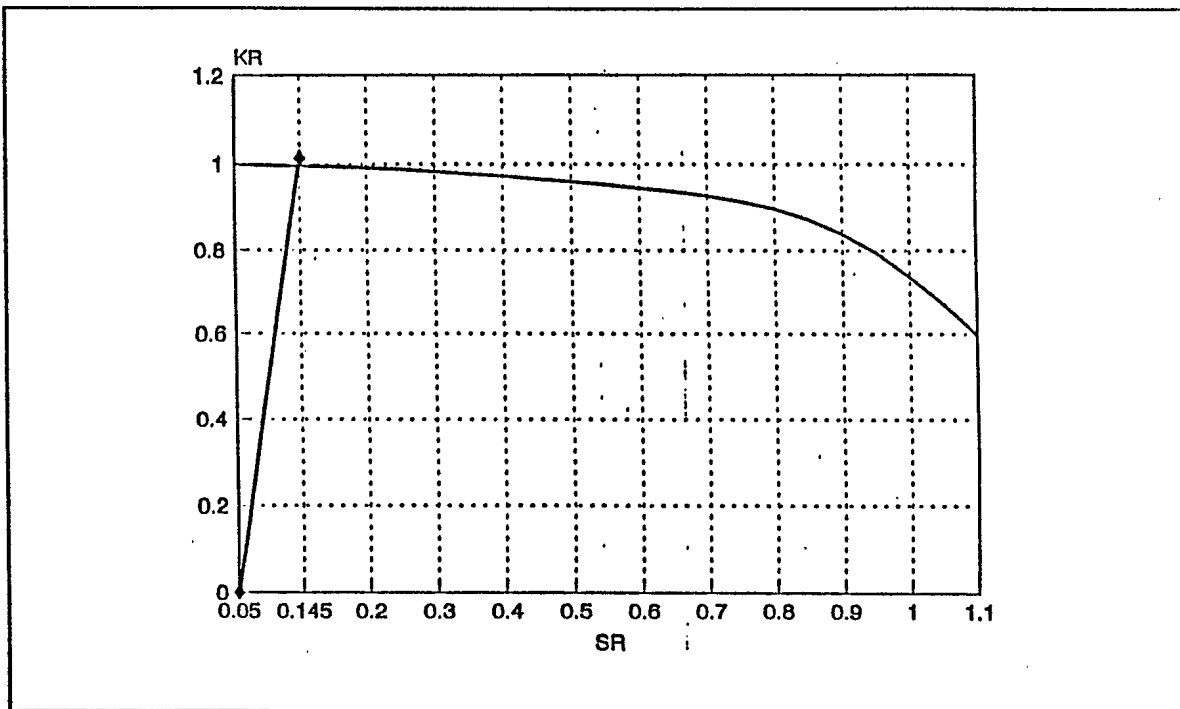
Figure 8. Failure Assessment Diagram from PC-FAD
