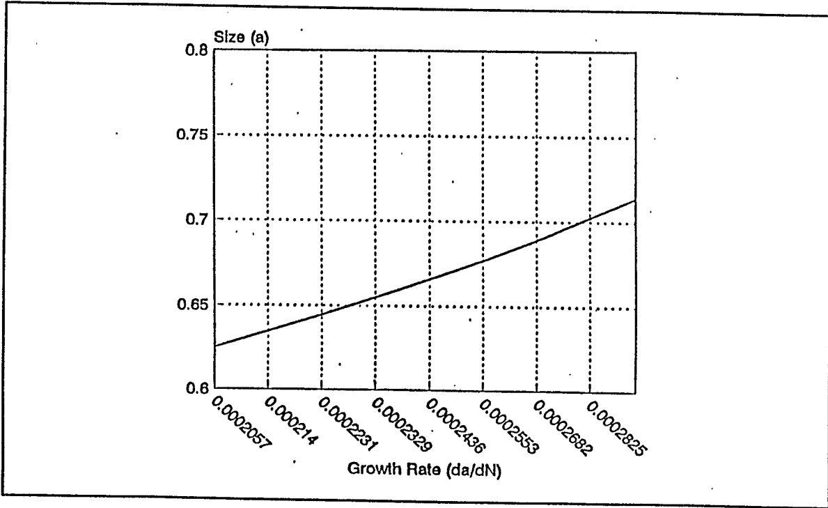
Figure 2. Crack Length vs Growth Rate for NASCRAC
