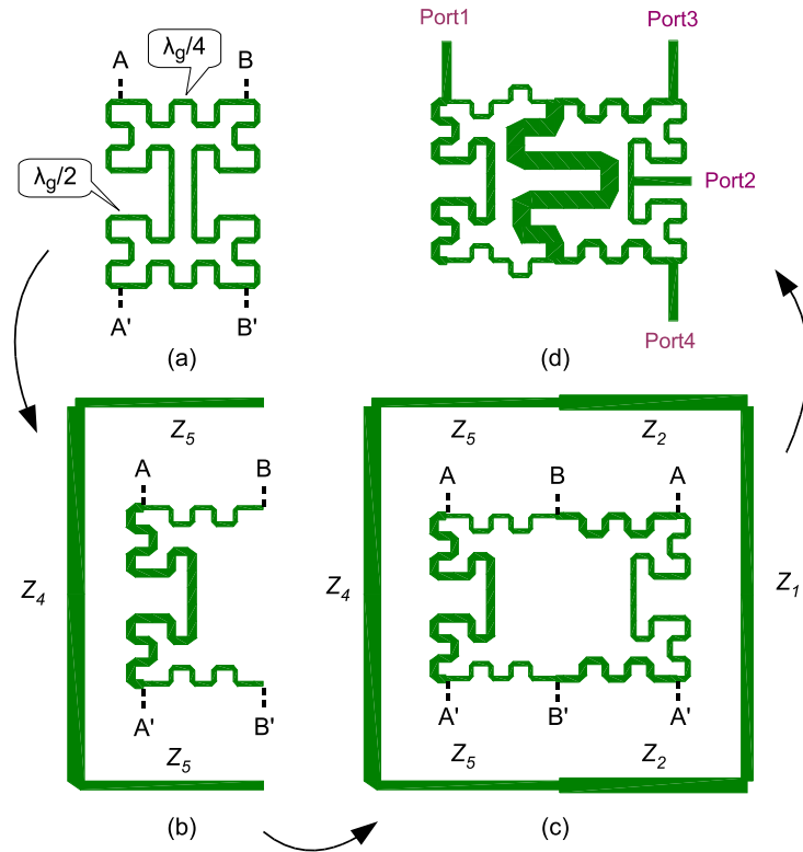
Figure 5: Implementation of the miniaturized broadband two-section 180^\circ hybrid from the fractal hybrid. (a) AB and AA' fractal hybrid curves are used as \lambda_g/4 and \lambda_g/2 lines, respectively. (b) The first section is constructed by connecting Z_4 and Z_5 lines. (c) Following the same procedure, the second section is then built by assembling Z_1 and Z_2 lines. (d) Finally, the central line Z_3 is meandered in the room in the middle of the two sections and ports are placed to complete the implementation.
