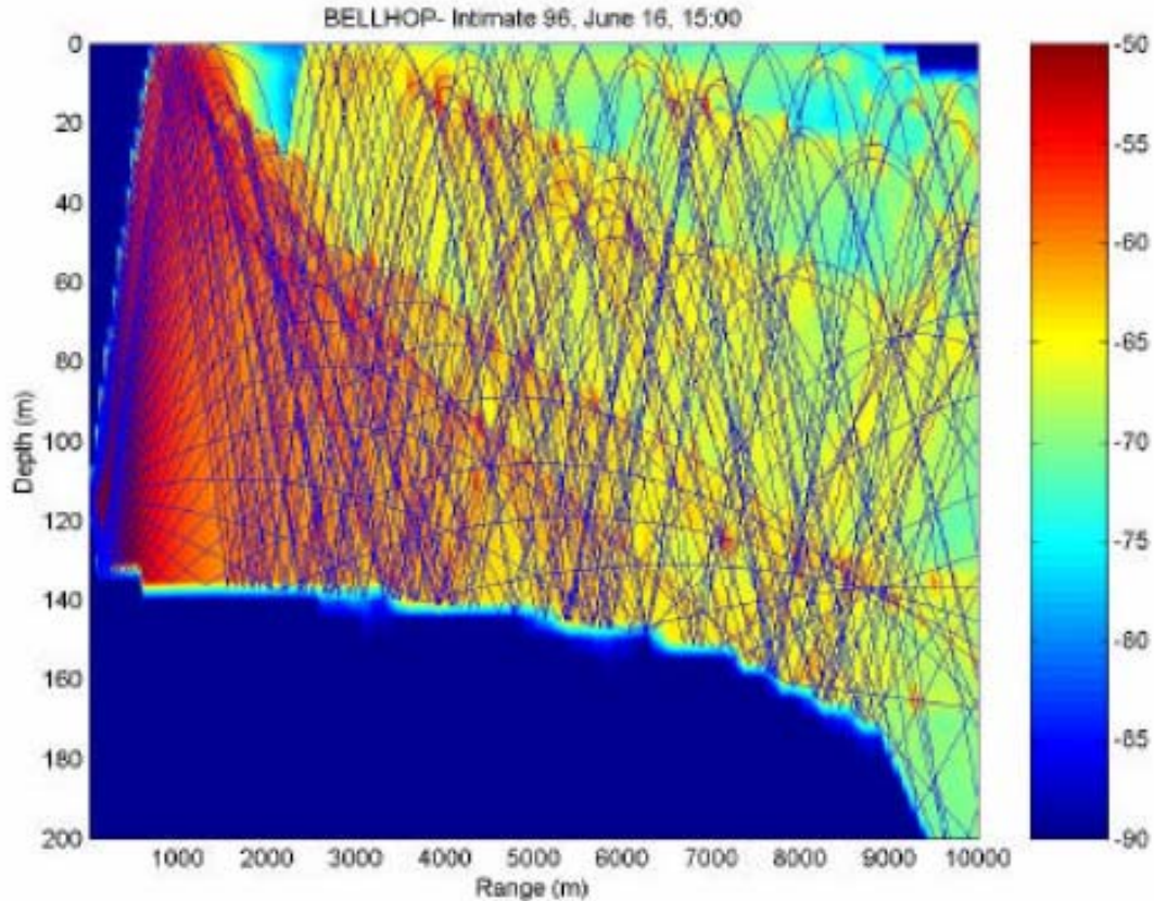
Figure 9. Combined Ray-Plot and Propagation Loss Display
