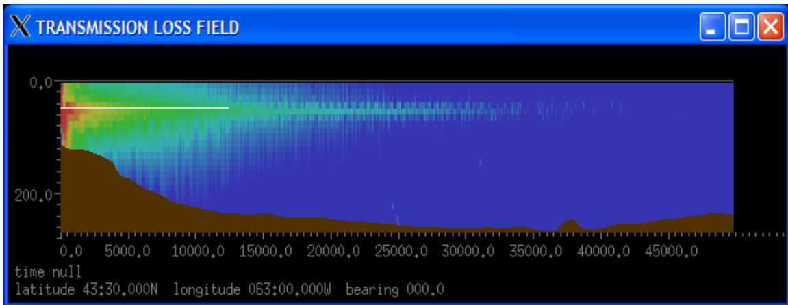
Figure 6. Transmission Loss vs. Range and Depth Display
