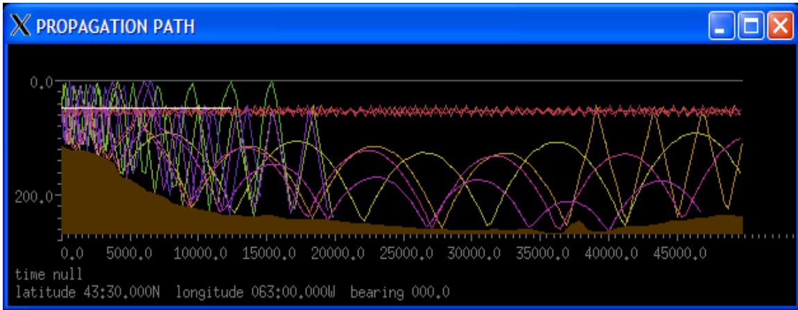
Figure 5. Propagation Ray Path Display
