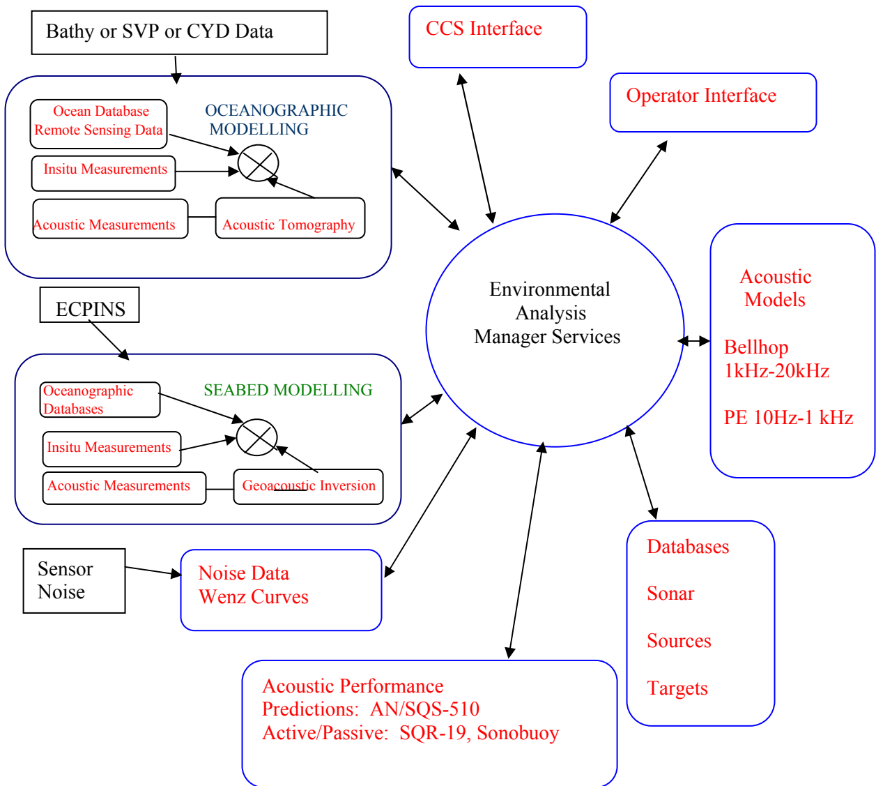
Figure 10. Advanced Environmental Analysis Package
