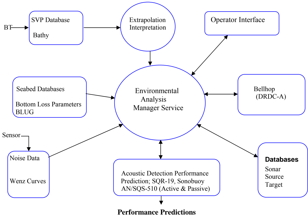
Figure 3. The Data-flow Structure for the NUW Developed Environmental Analysis Package
