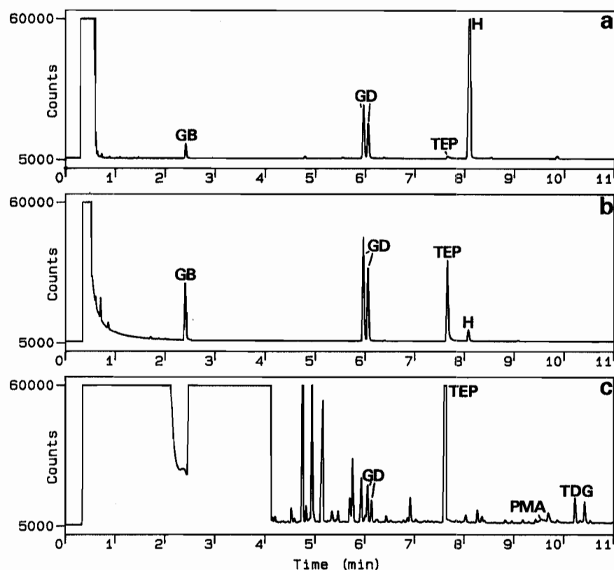
Fig. 2. Capillary column gas chromatograms of successive extraction of 50 µg/g of sarin (GB), soman (GD), triethyl phosphate (TEP) and mustard (H) added to loamy sand with (a) hexane, (b) dichloromethane and (c) TMS derivatizing agent. TDG = di-TMS derivative of thiodiglycol; PMA = TMS derivative of pinacolyl methylphosphonic acid. For conditions, see text.
