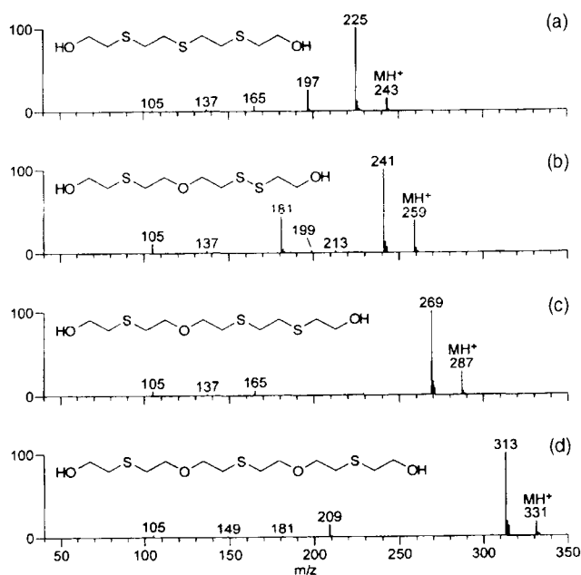
Fig. 4. ESI-MS/MS product mass spectra obtained for the [M+H]^+ ion of (a) 3,6,9-trithia-1,11-undecanediol (collision energy: 5 V), (b) 6-oxa-3,9,10-trithia-1,12-dodecanediol (collision energy: 5 V), (c) 6-oxa-3,9,12-trithia-1,14-tetradecanediol (collision energy: 5 V) and (d) 6,12-dioxo-3,9,15-trithia-1,17-heptadecanediol (collision energy: 7 V) during LC-ESI-MS/MS analysis of an aqueous extract of a soil sample taken from a former mustard storage site.
