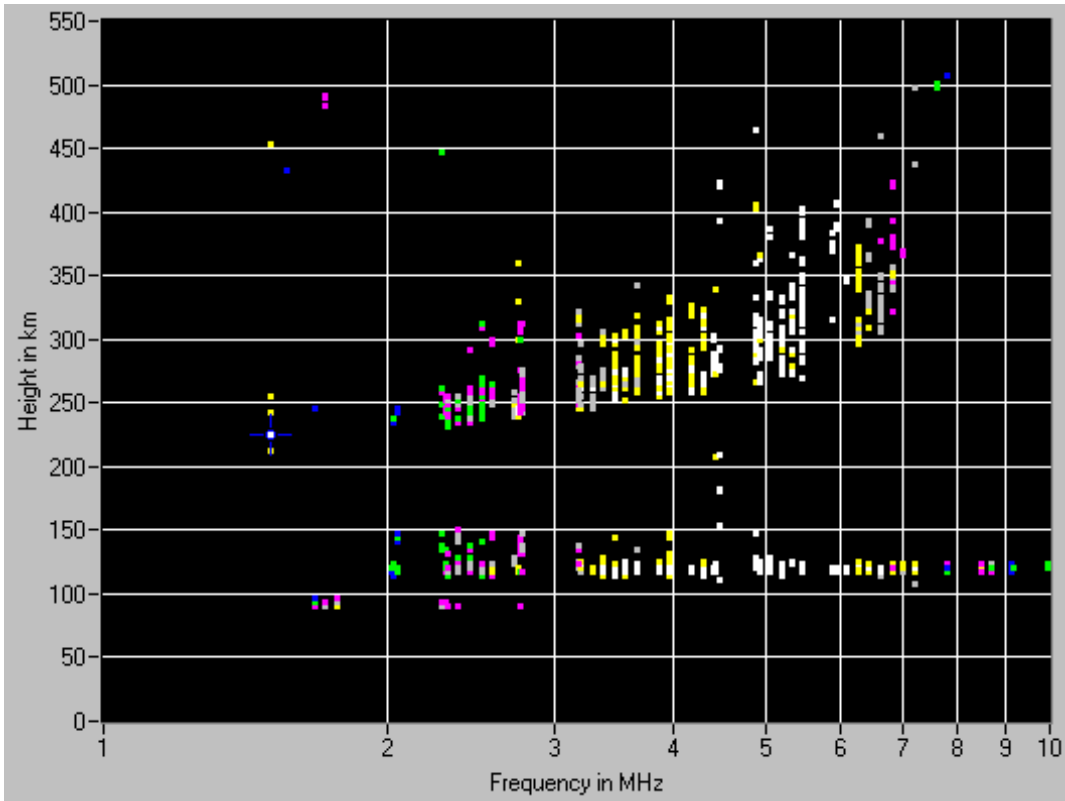
Figure 4: Height-spread sporadic E; taken on August 28, 2000, hour 02:00 UT at Cape Race.
