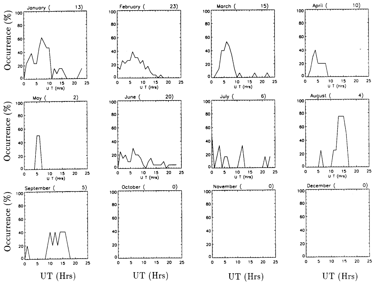
Figure 9: Occurrence statistics for the height-spread Es for the year 1998 at Cambridge Bay. The number of days of data collection is shown in brackets for each month.
