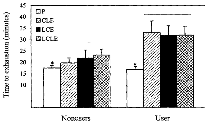
Fig. 1. Time to exhaustion (mean ± SEM) in caffeine users and nonusers after ingesting different doses of caffeine plus ephedrine. p = placebo; CLE = 5 mg · kg -1 C + 0.8 mg · kg -1 E, LCE = 4 mg · kg -1 C + 1 mg · kg -1 E, LCLE = 4 mg · kg -1 C + 0.8 mg · kg -1 E *P similar in users and nonusers and significantly different from C+E trials. Lines represent similar means Users significantly different from nonusers for the C+E treatment trials.
