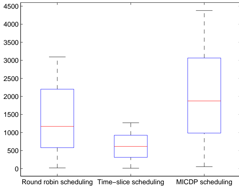
Figure 23: Total number of Discrimination Conflicts ( DC_{[1,\dots,15]} )
