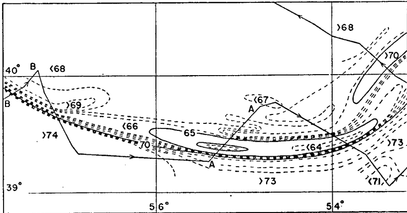
Figure 2. Surface temperature contour plot from STD data of H. M. C. S. NEW LISKEARD . Ship's course is shown as arrowed lines. Sections AA and BB cross the Stream at an angle of about 60^{\circ} to the current which parallels the isotherms.
