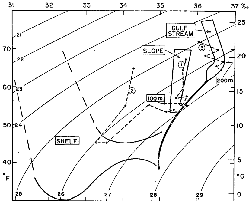
Figure 6. T-S envelopes of Gulf Stream, Slope and Shelf waters. Surface layer Shelf water is shown dashed. Curves 1, 2 and 3 are those of Fig. 4, indicating cold water of No. 2 to be of Shelf water origin.
