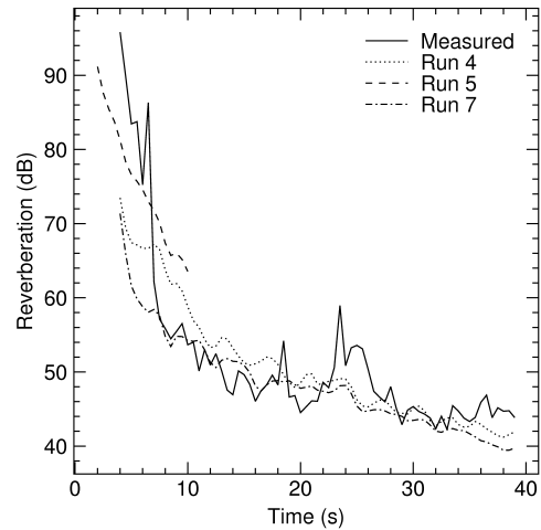
Figure 4. Beam 2 – 090.8° T
