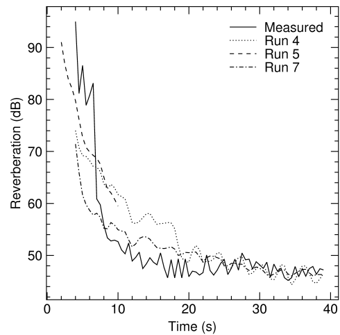
Figure 6. Beam 4 – 276.2° T
