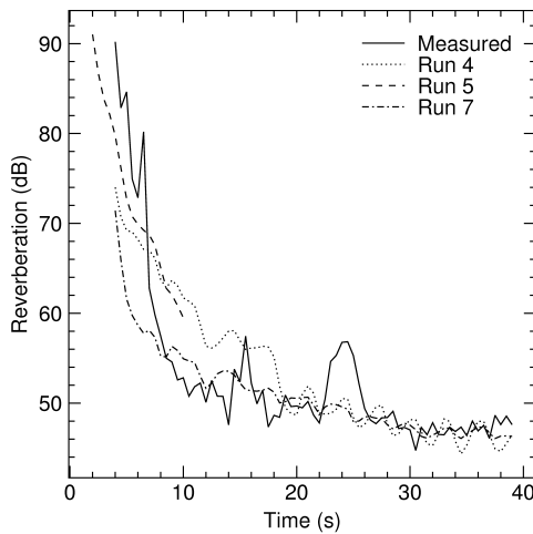
Figure 5. Beam 3 – 119.8° T
