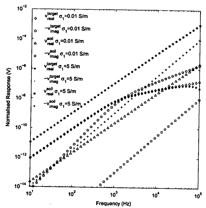
Fig. 8. Response of a buried spherical target for two values of soil conductivity (0.01 and 5 S/m). Response of the soil alone is also plotted for comparison. Sensor standoff h = 0 m, object depth d = 0.1 m, soil susceptibility \chi_0 = 0 .
