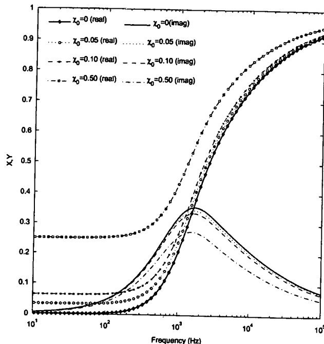
Fig. 4. Effect of frequency-independent soil on the response functions of an aluminum sphere of radius R = 0.005 m, conductivity \sigma_2 = 3.54 \times 10^7 S/m.
