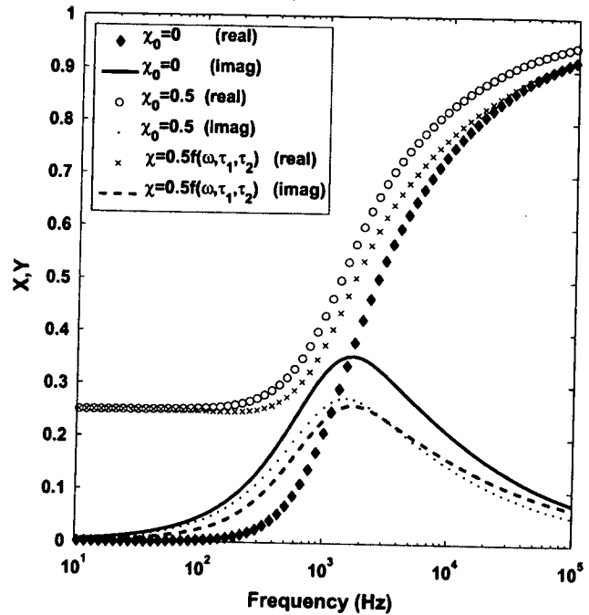
Fig. 6. Effect of soil with frequency-dependent susceptibility compared with that of frequency-independent soil on the response functions of an aluminum sphere of radius R = 0.005 m, conductivity \sigma_2 = 3.54 \times 10^7 S/m.
