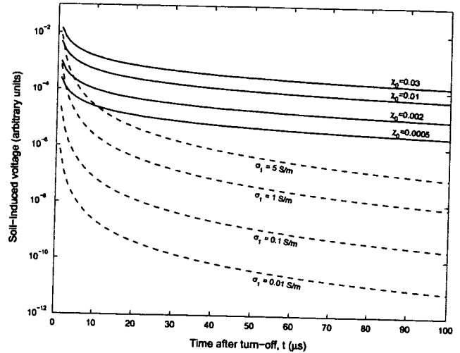
Fig. 3. Relative contributions of conductivity and frequency-dependent susceptibility to the signal produced by soil in a metal detector. Values of magnetic relaxation time constants used are \tau_1 = 10^{-6} s and \tau_2 = 10^{-3} s.
