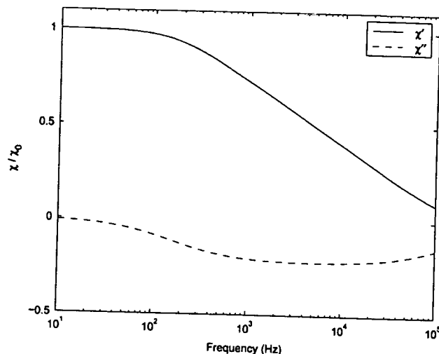
Fig. 2. Model for frequency-dependent soil susceptibility used in this paper. The real and imaginary parts of \chi are computed using (2) with \tau_1 = 10^{-6} s and \tau_2 = 10^{-3} s.
