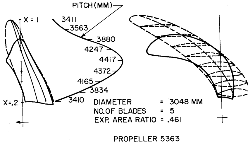
FIG. 5: GEOMETRY OF NEW PROPELLERS FOR QUEST.
