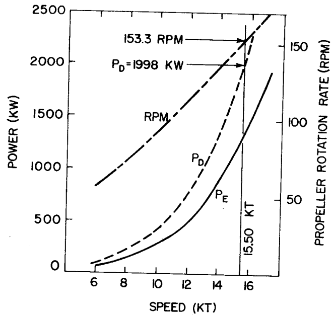
FIG. 3: PROPULSION TEST WITH STOCK PROPELLERS. DRAUGHT, 4650 MM.
