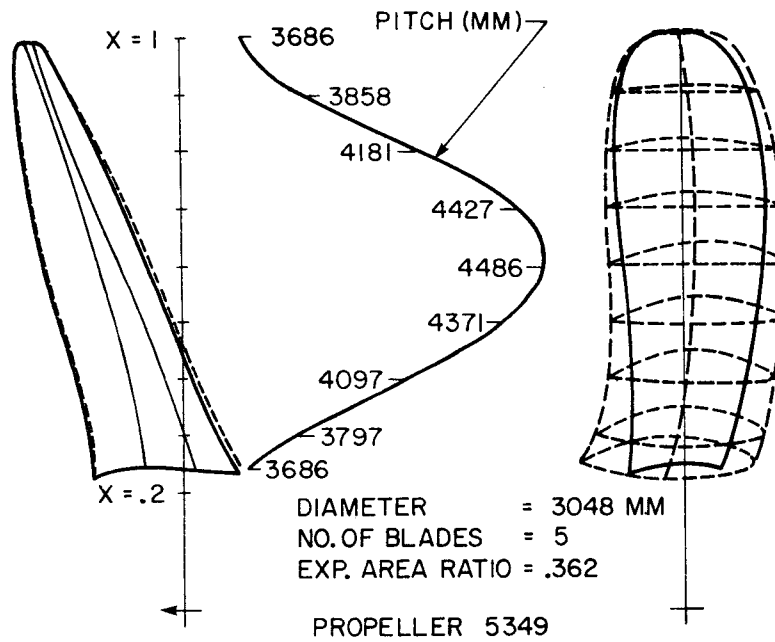
FIG. 2: GEOMETRY OF PRESENT PROPELLERS ON QUEST.
