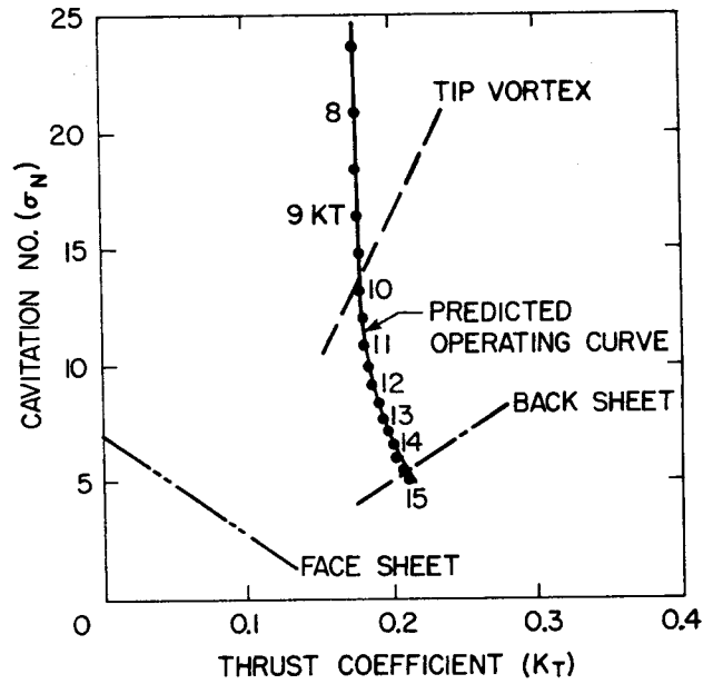
FIG. 10: CAVITATION INCEPTION, PROPELLER 5363, BEHIND CONDITION. DRAUGHT, 4650 MM.
