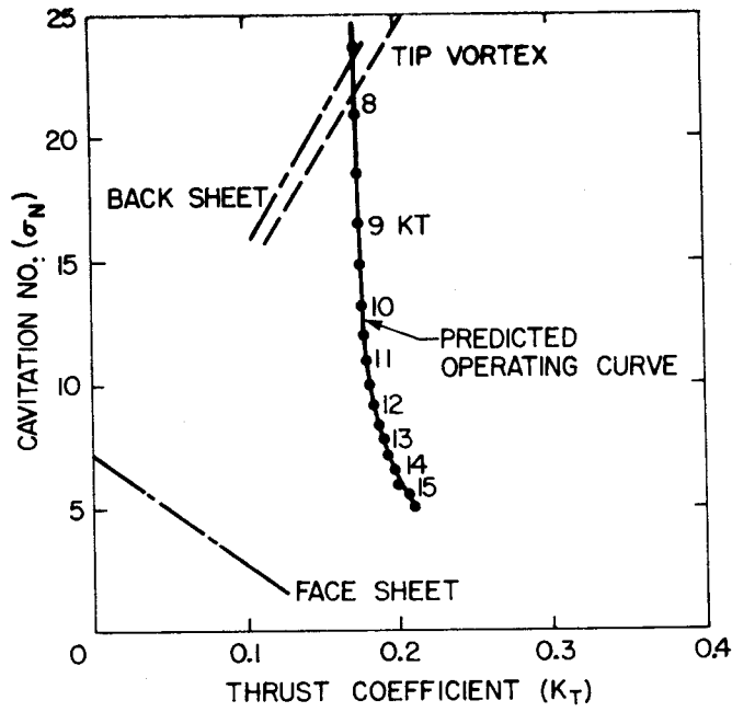
FIG. 9: CAVITATION INCEPTION, PROPELLER 5349, BEHIND CONDITION. DRAUGHT, 4650 MM.
