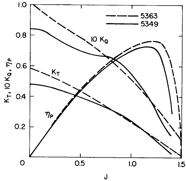
FIG. 7: MEASURED OPEN WATER DATA FOR PROPELLERS 5349 AND 5363.
