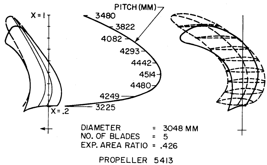
FIG. 16: GEOMETRY OF NEW PROPELLERS FOR A-BRACKET CONFIGURATION.
