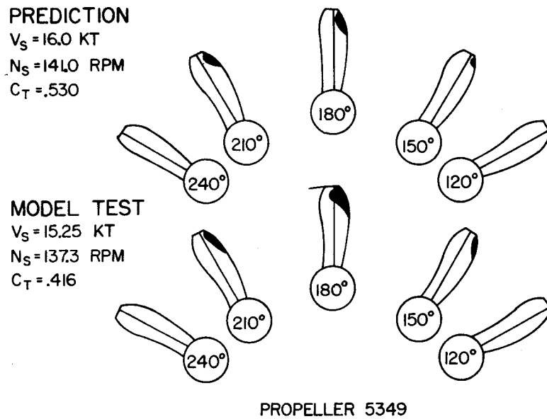
FIG. 12: CALCULATED AND MEASURED SUCTION-SIDE CAVITATION PATTERNS, PROPELLER 5349.
