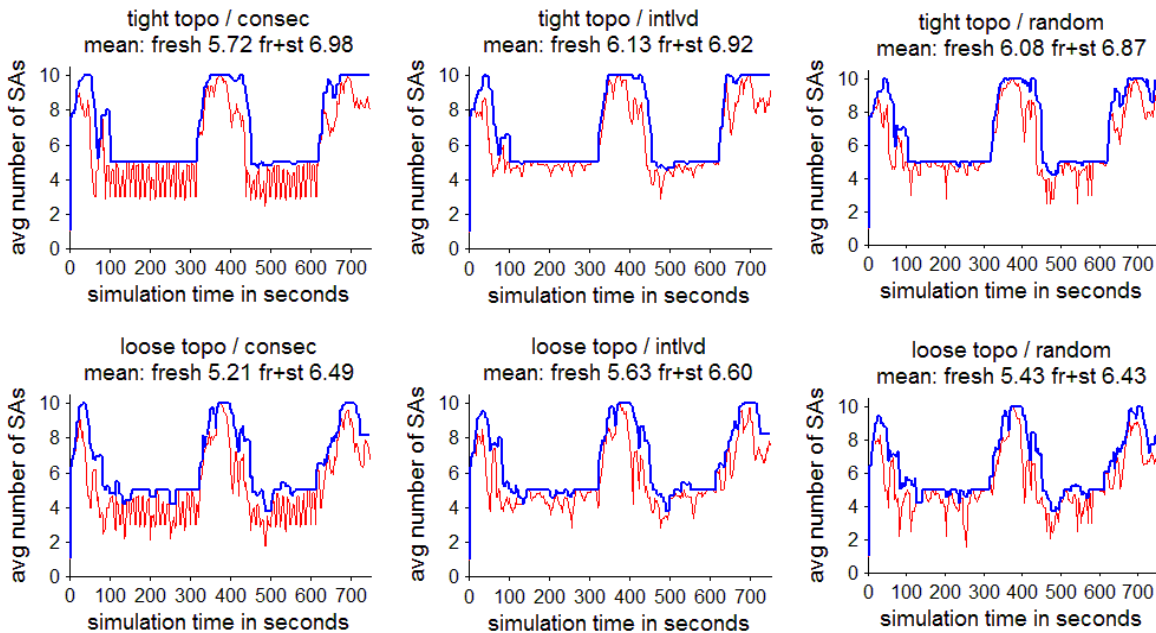
Figure 5: Average SA count – Fresh \bar{N}_{fr} (in red) and Fresh-plus-Stale \bar{N} (in blue) for tight topology (above) and loose topology (below) in three different flooding orders.
