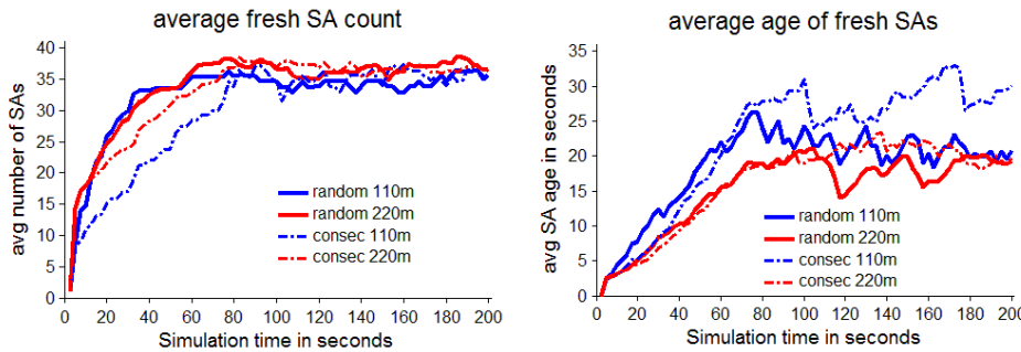
Figure 3: Comparison of average SA count and age in different flooding orders and radio ranges.
