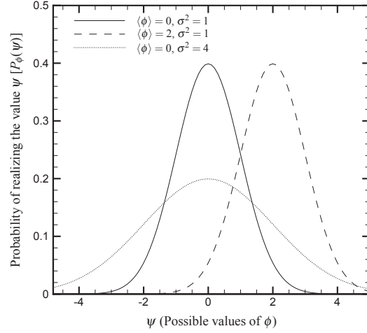
Figure 1: Gaussian probability distribution function
