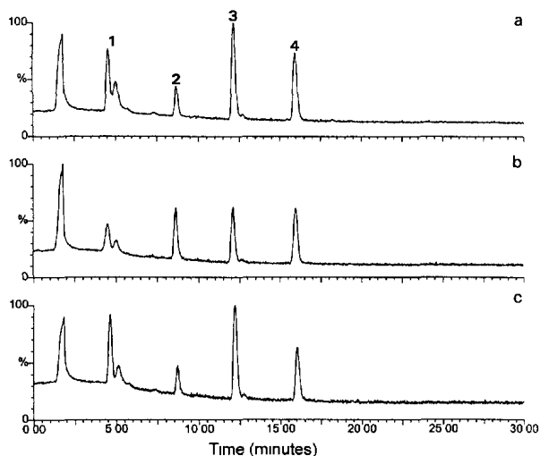
Fig. 3 Packed capillary LC–ESI–MS total ion current ( m/z 400 to m/z 85) chromatograms obtained for an aqueous extract of (a) red clay, (b) tan sandy clay and (c) brown sandy clay loam soil samples spiked at the 10 \mu\text{g/g} level with isopropyl methylphosphonic acid (1), sarin (2), pinacolyl methylphosphonic acid (3) and soman (4)
