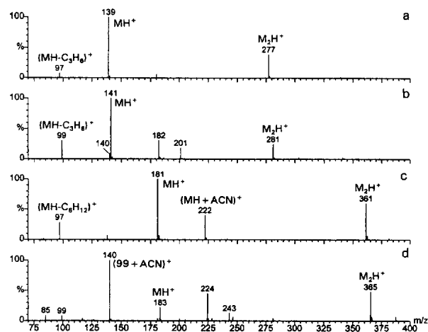
Fig 4 Typical ESI–MS data (sampling cone voltage 20 V) obtained for (a) isopropyl methylphosphonic acid, (b) sarin, (c) pinacolyl methylphosphonic acid and (d) soman during analysis of aqueous soil extracts
