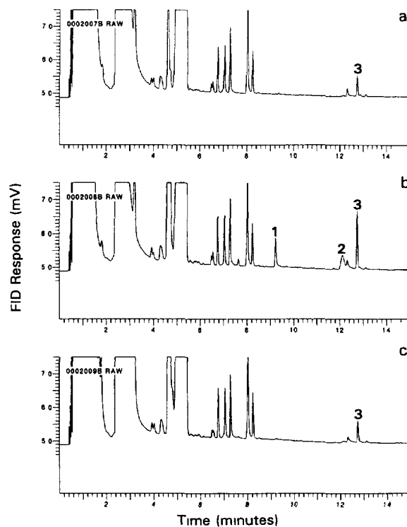
Fig 2 Capillary column GC–FID chromatograms obtained for trimethylsilyl/dichloromethane extract of (a) red clay, (b) tan sandy clay and (c) brown sandy clay loam soil samples spiked at the 50 µg/g level with isopropyl methylphosphonic acid (1), pinacolyl methylphosphonic acid (2) and thiodiglycol (3).
