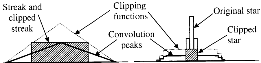
Fig. 5. Shape of the objects (star and streak), their convolution peaks and clipping functions.
