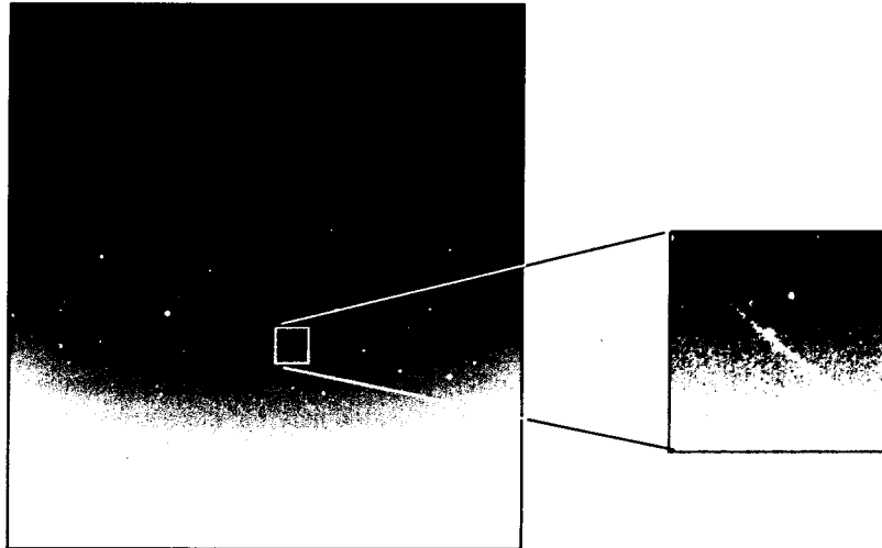
Fig. 2. An example of an image acquired for the detection of a satellite.
