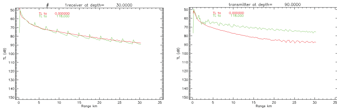
Figure 4. Left: TL from receiver to surface (red) and bottom (green). Right: TL from source to surface (red) and bottom (green).
