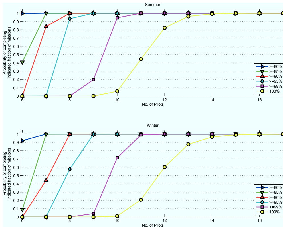
Figure 15: Probability of meeting manning requirements for 12/5 operations in 6-month deployment of 6 aircraft with aircraft serviceability rates of 70% and 50% as a function of total aircrew.
