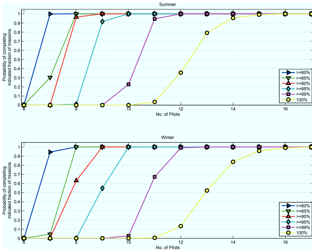
Figure 16: Probability of meeting manning requirements for 12/5 operations in 6-month deployment of 6 aircraft with aircraft serviceability rates of 70% and 70% as a function of total aircrew.
