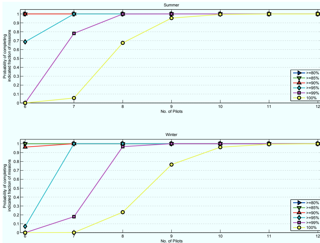
Figure 8: Estimated probability of meeting manning requirements for a 6 month deployment of 6 CF188 with continuous 12/5 operations as a function of total number of aircrew, aircrew illness parameters and percentage of planned sorties completed. Daily aircrew demand is fixed at 6. The minimum manning requirement is 6 crews.
