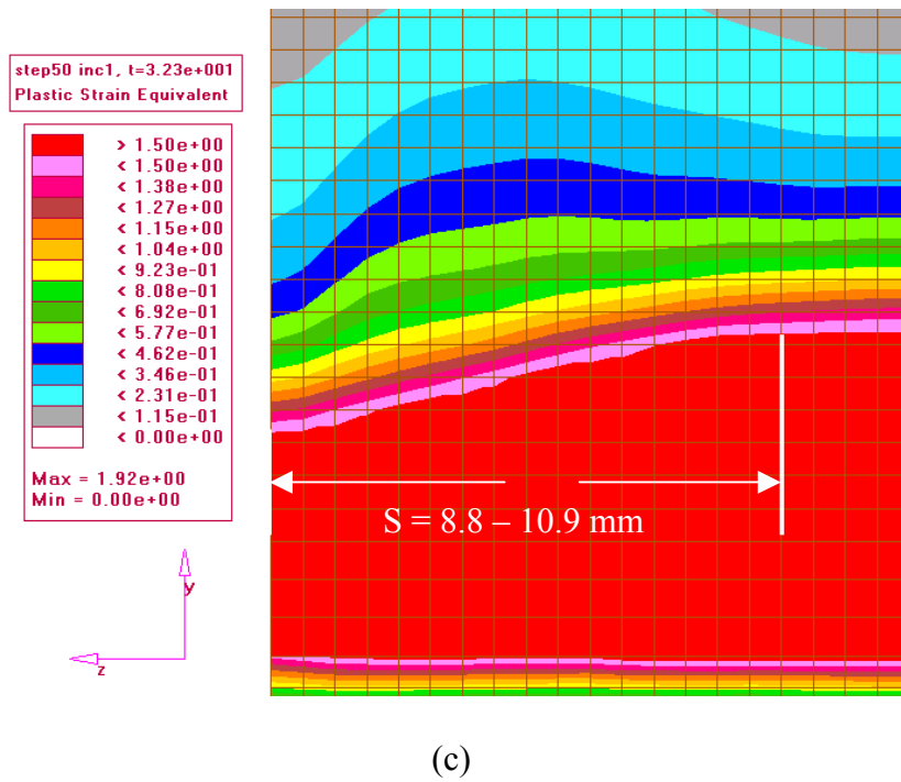
Figure 4.11: (a) Plastic Strain Contours, (b) Crack Propagation and (c) Close-up View of Plastic Strain Contours for Model With Curve 3 Material Properties Using Plastic Strain as Removal Criterion ( a/W = 0.45 )
